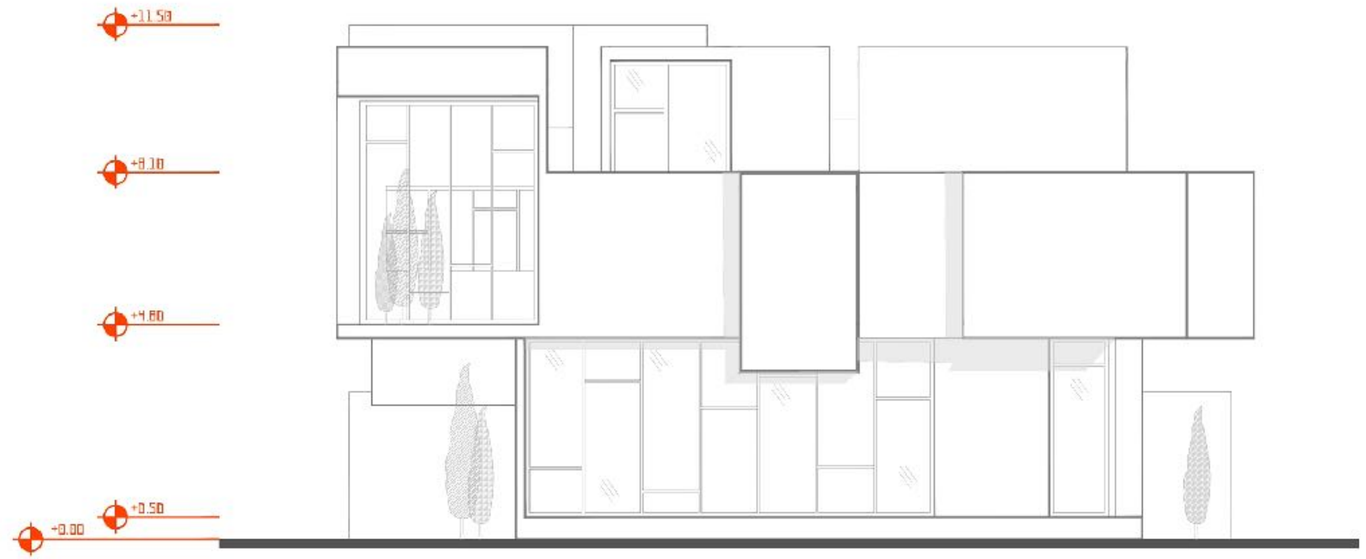
4 N Facad Scale 1:100
