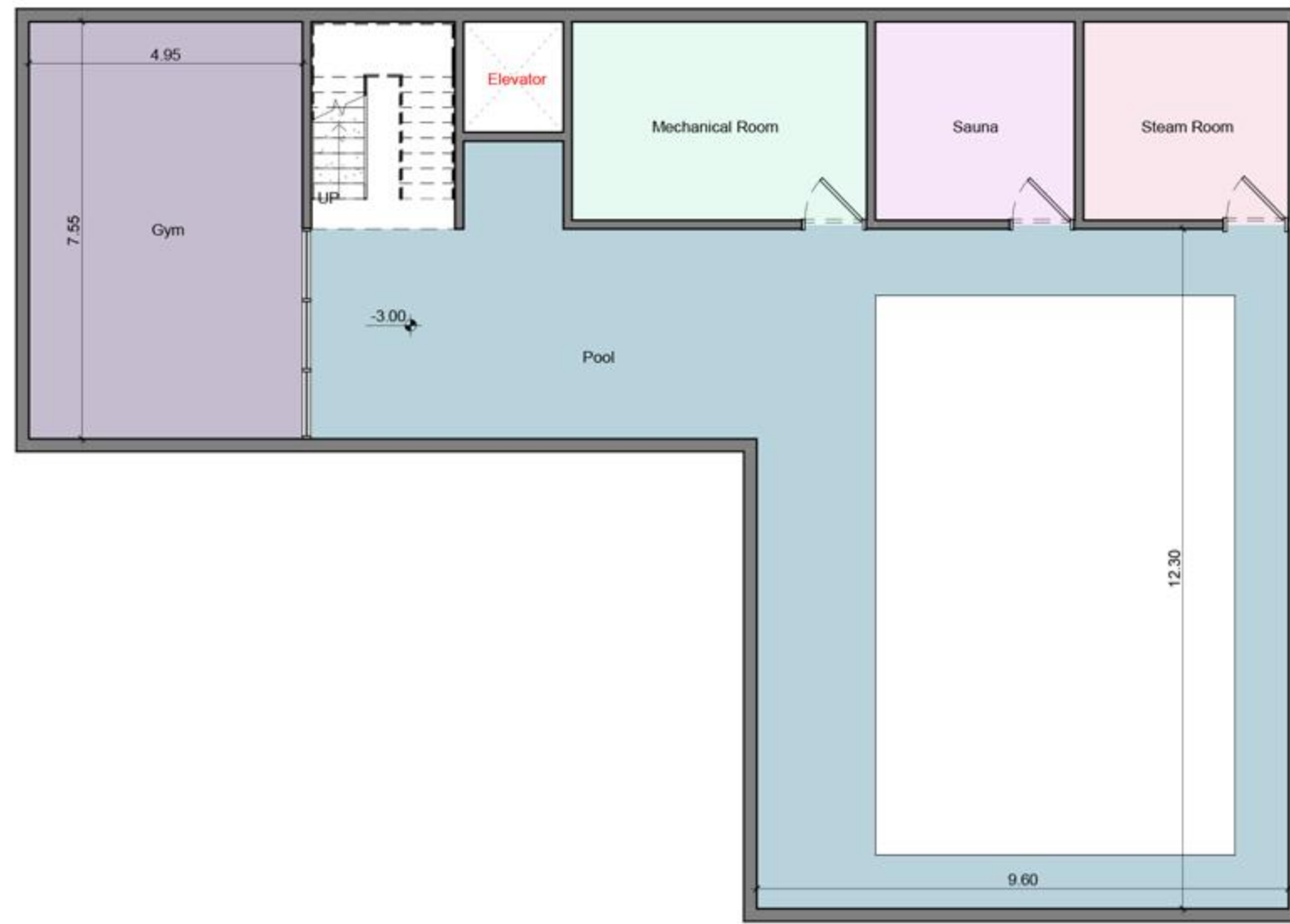
1 First Basement Floor 1:100
