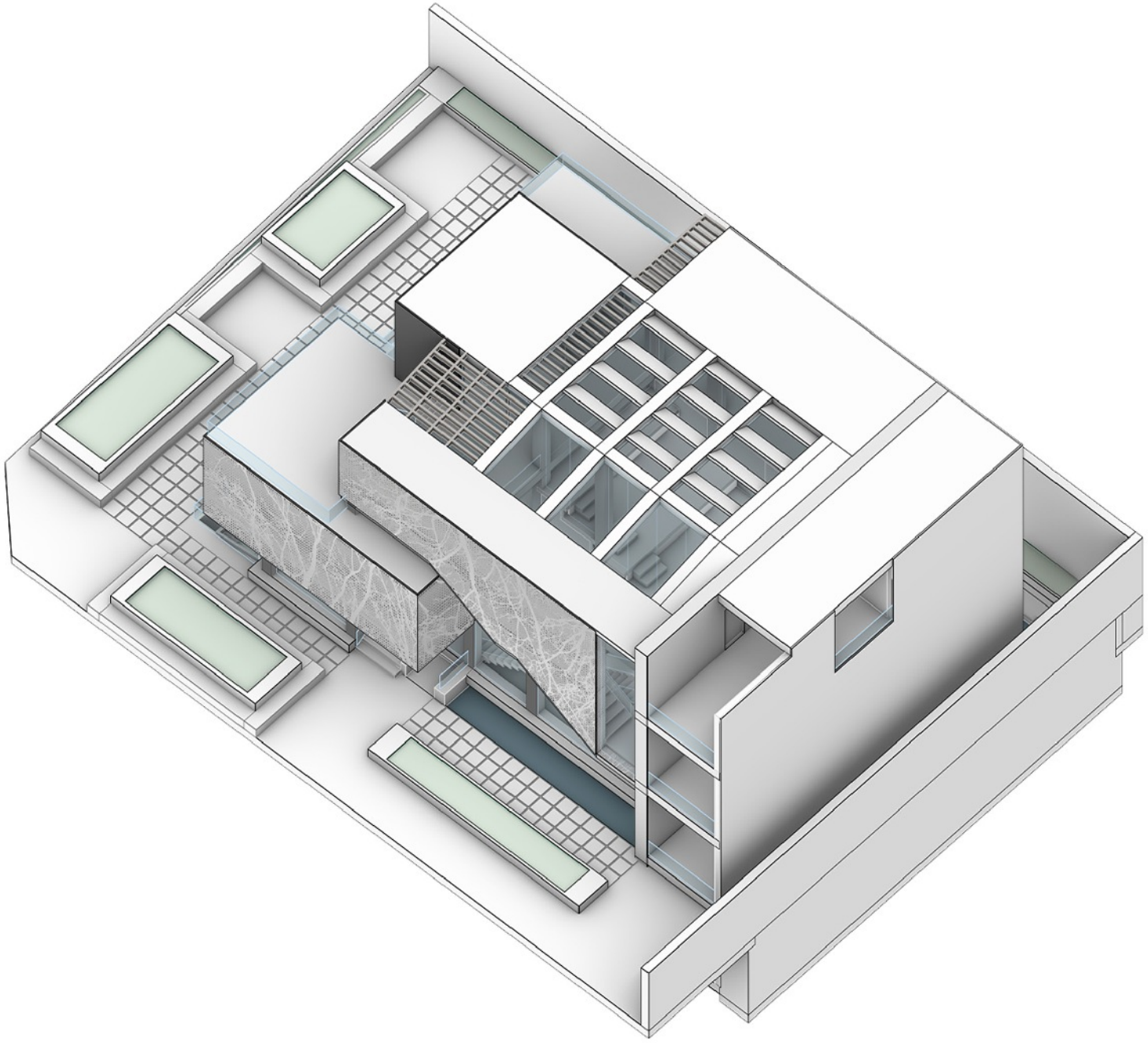
Roof Plan
