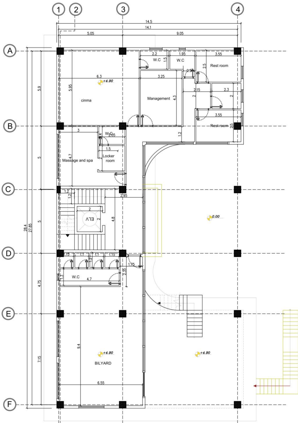
First Floor Plan SC:1:100
