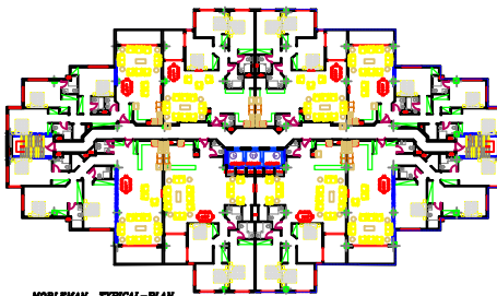
NOBLEMAN TYPICAL-PLAN 2APF
