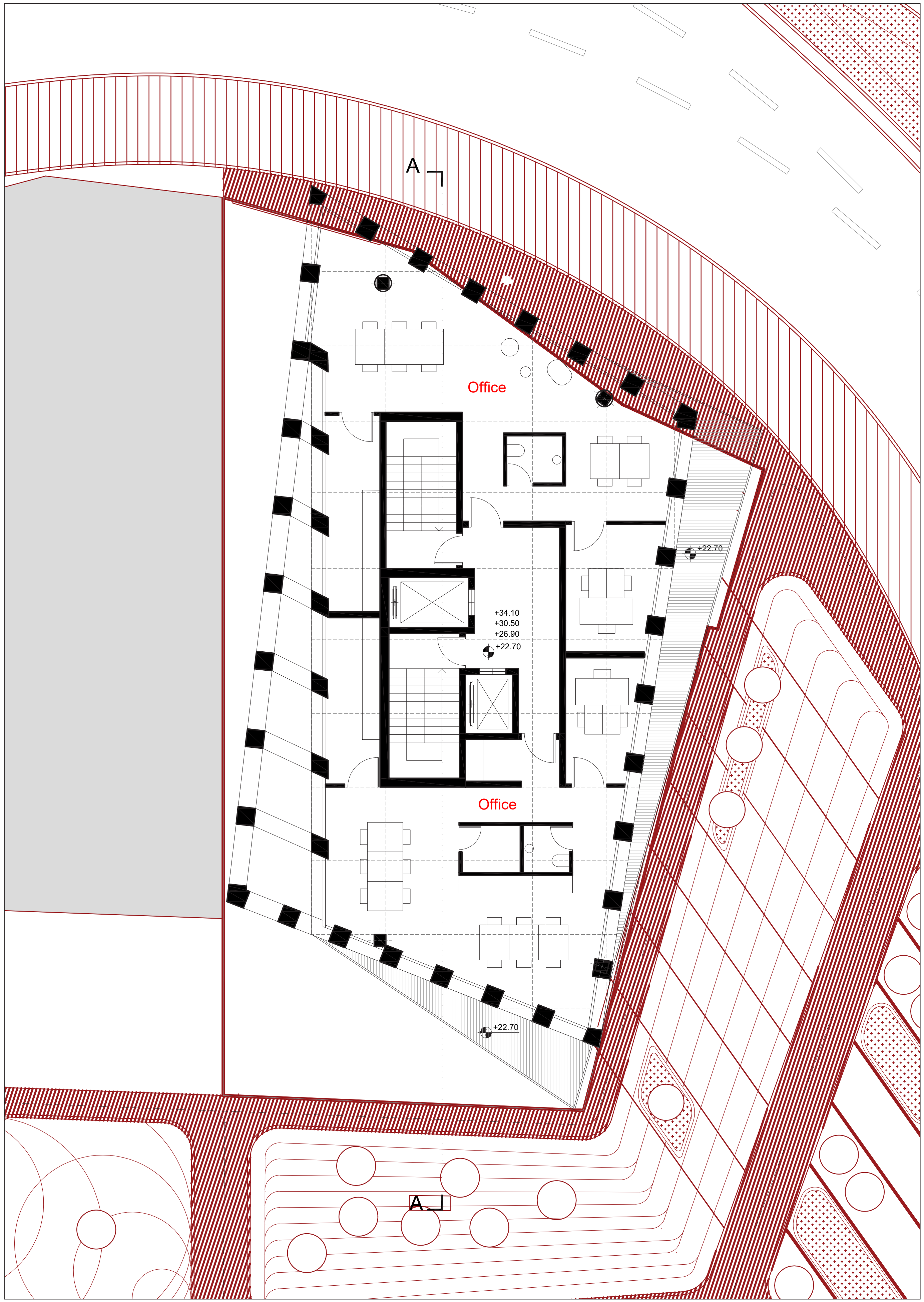
5th-8th Floor Plan S.c 1:100 Level: -
