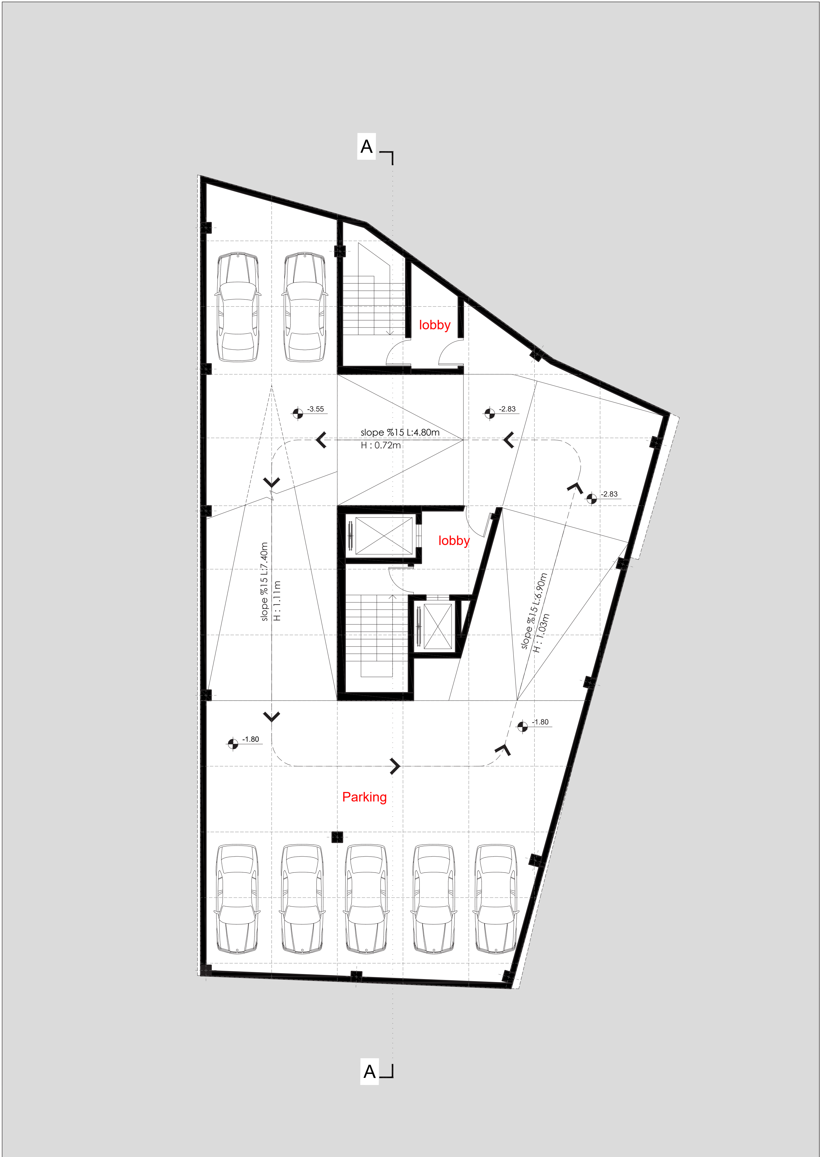
Basement -1 S.c 1:100 Level :-
