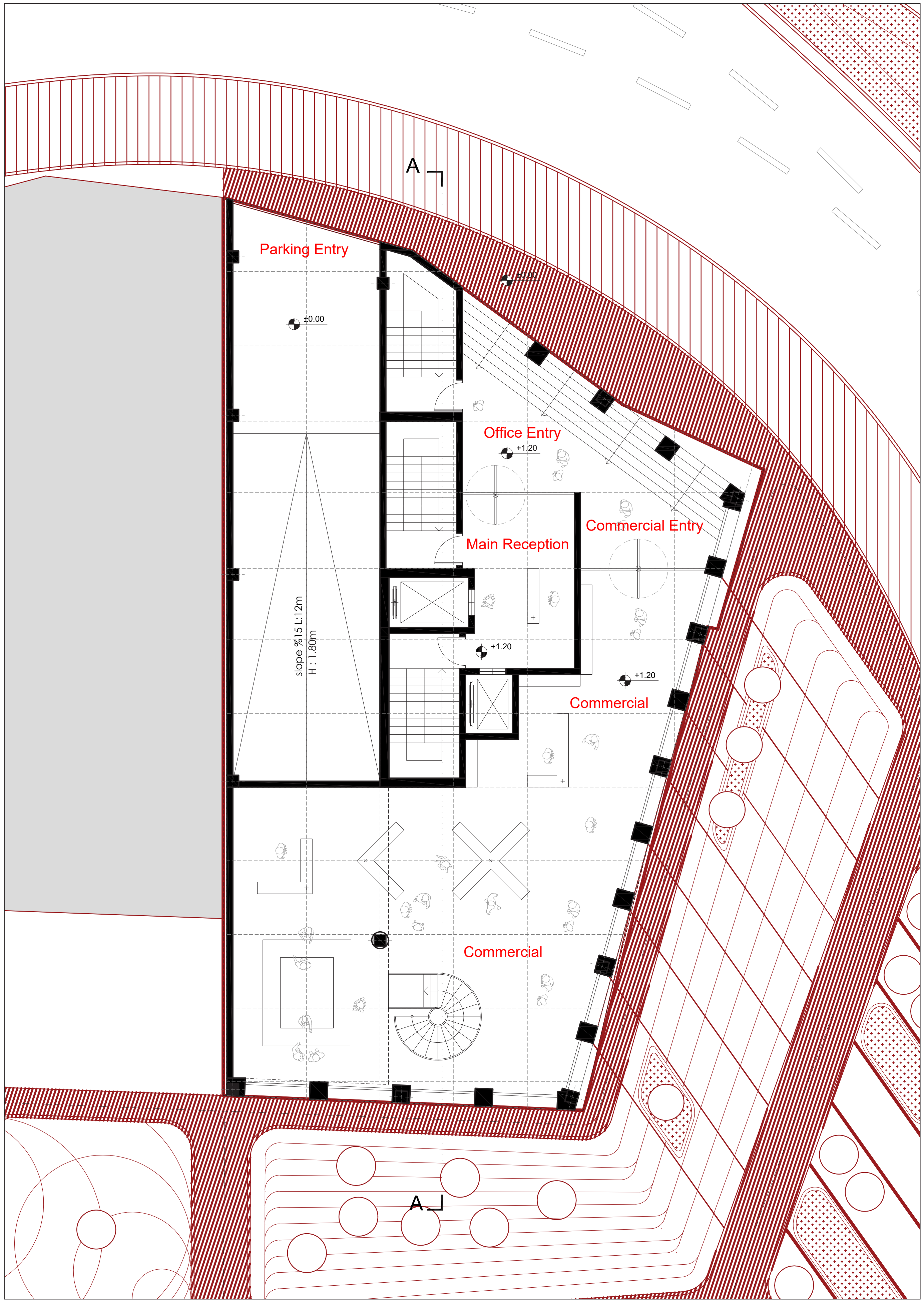
Ground Floor Plan s.c 1:100 Level : +1.20
