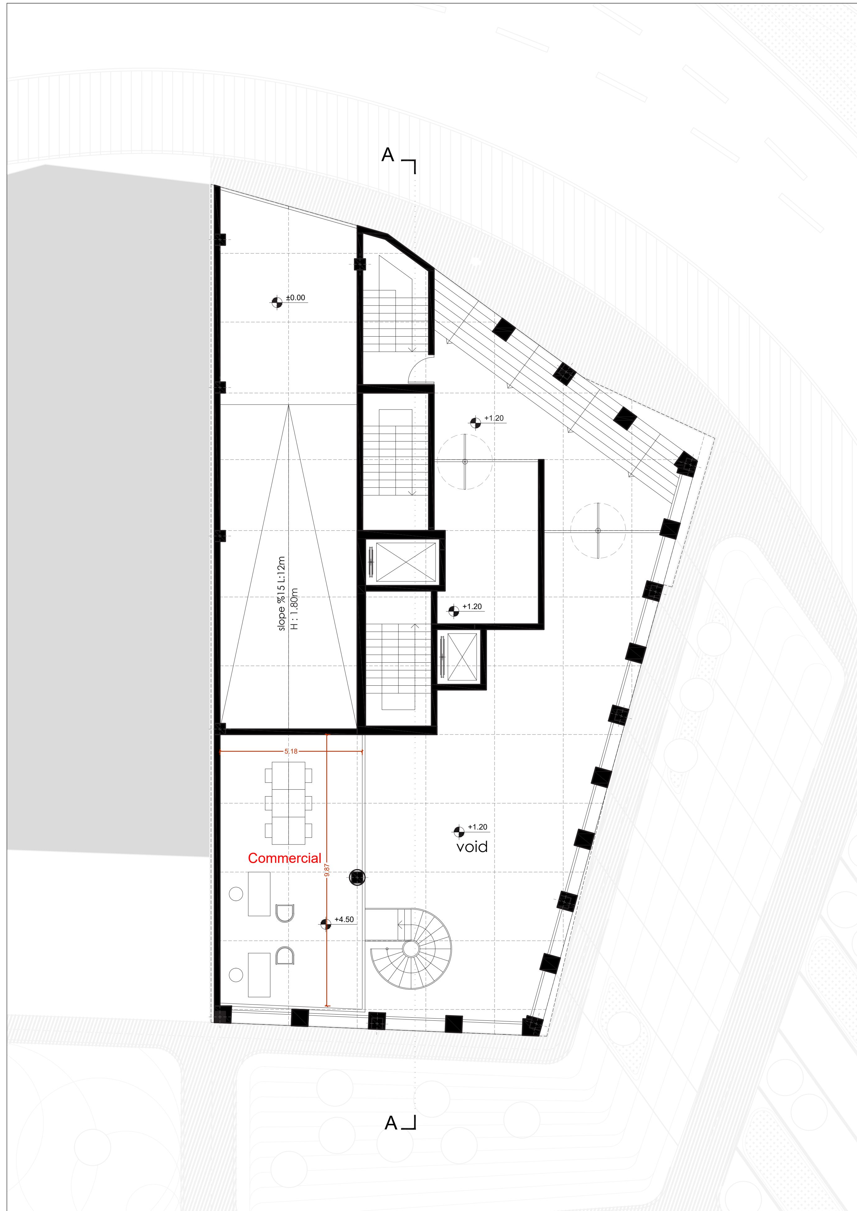
Mezzanine Floor Plan S.c 1:100 Level: +4.50
