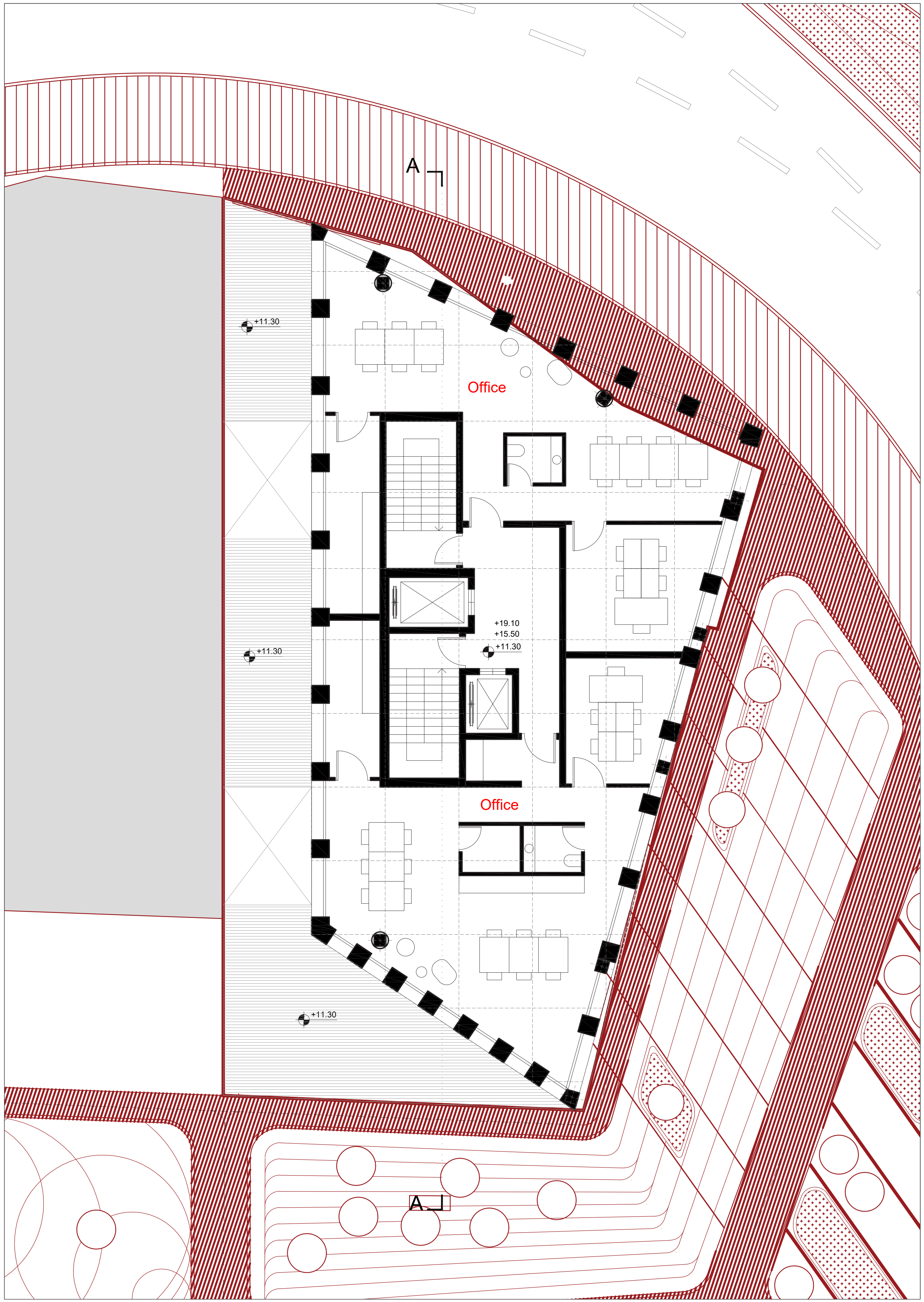
2th-4th Floor Plan s.c 1:100 Level :-
