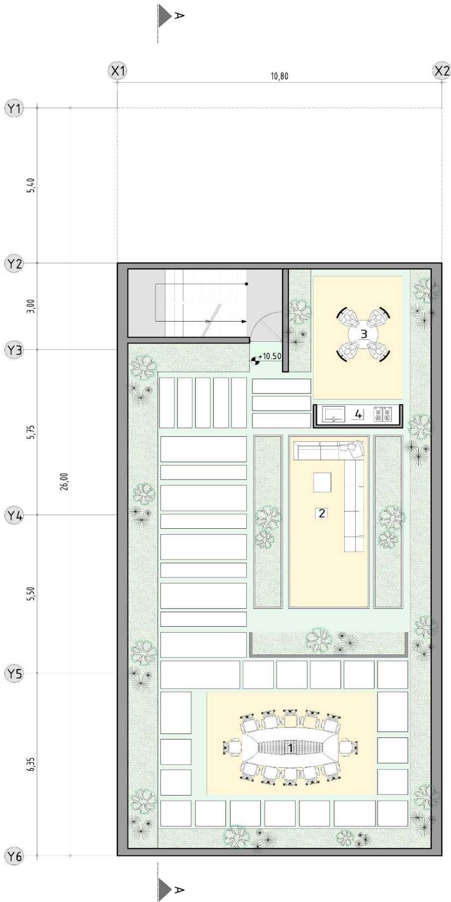
ROOF GARDEN PLAN
