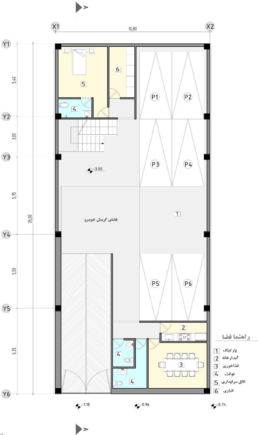
PLAN BASMENT -1
