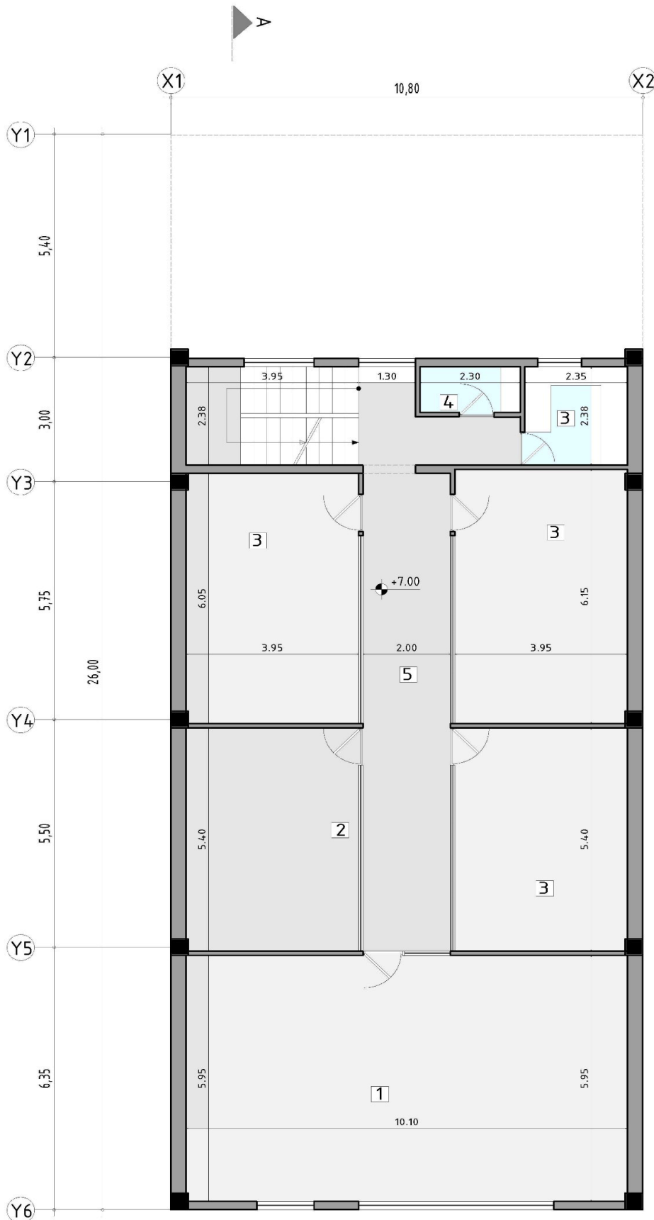
DIMENSION FLOOR PLAN 1
