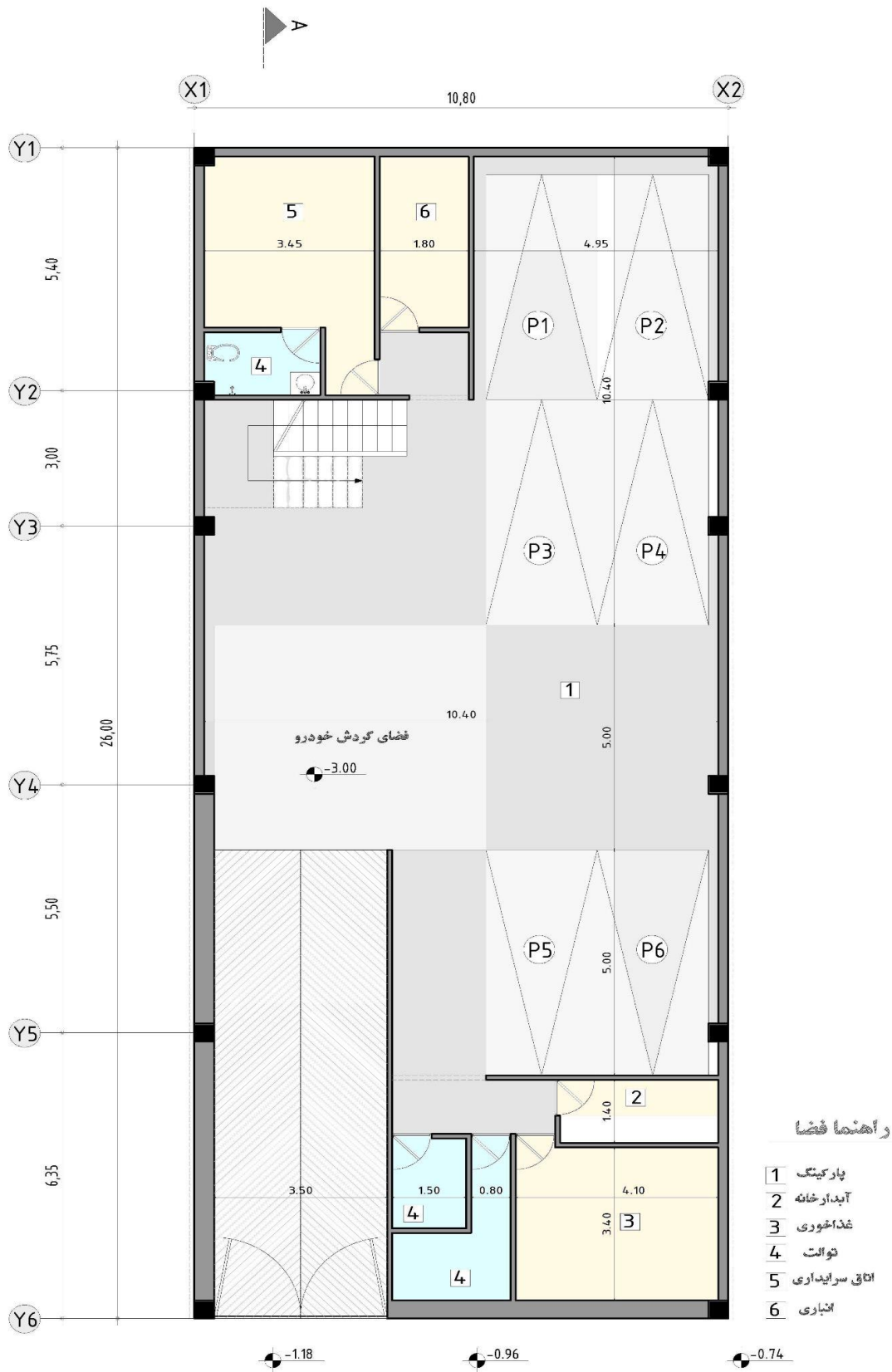
DIMENSION PLAN BASMENT -1
