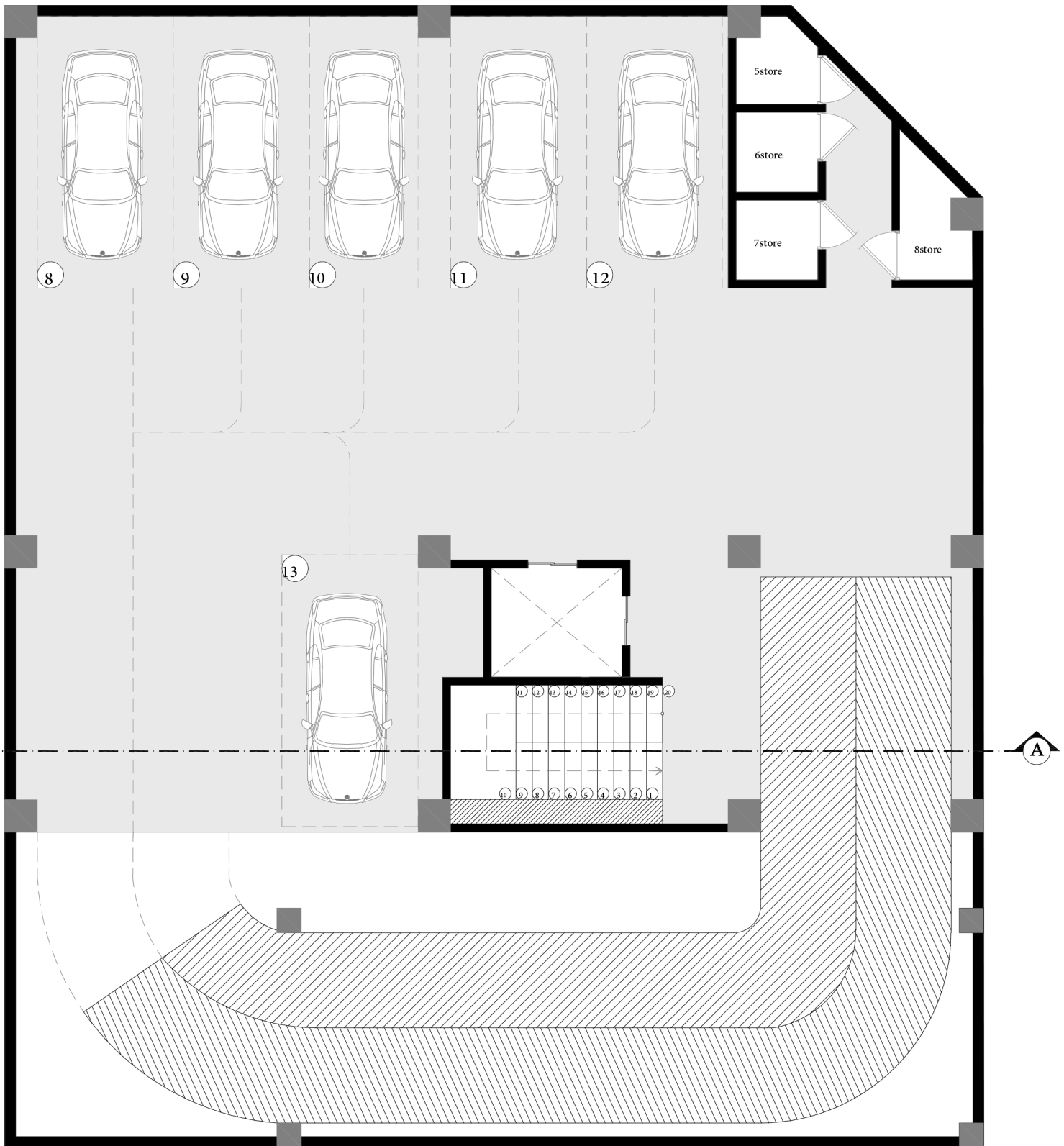
plan -1
