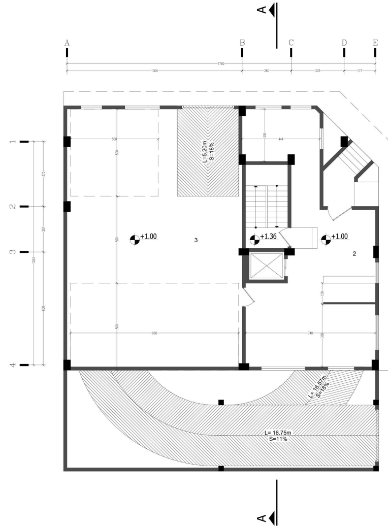
GROUND FLOOR (DIMENTION)
