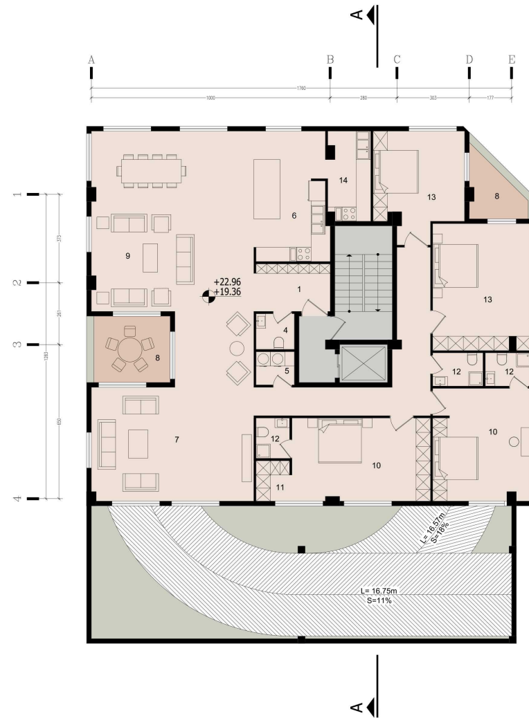
5 & 6 FLOOR (FURNITURE)
