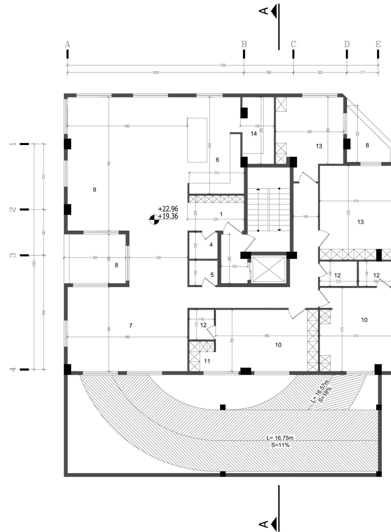
5 & 6 FLOOR (DIMENTION)
