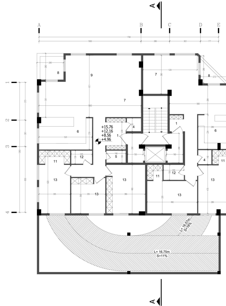
1 - 4 FLOOR (DIMENTION)
