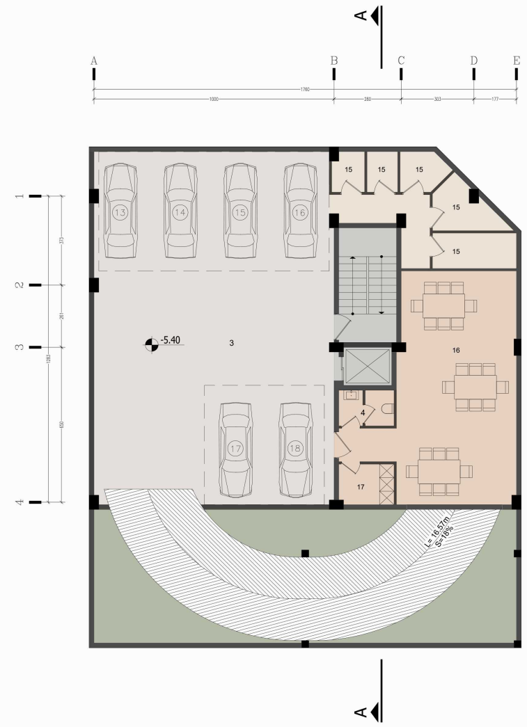
-2 PLAN (FURNITURE)
