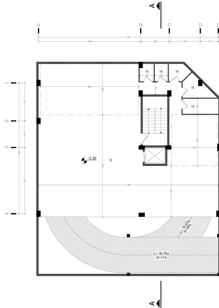
-1 PLAN (DIMENTION)
