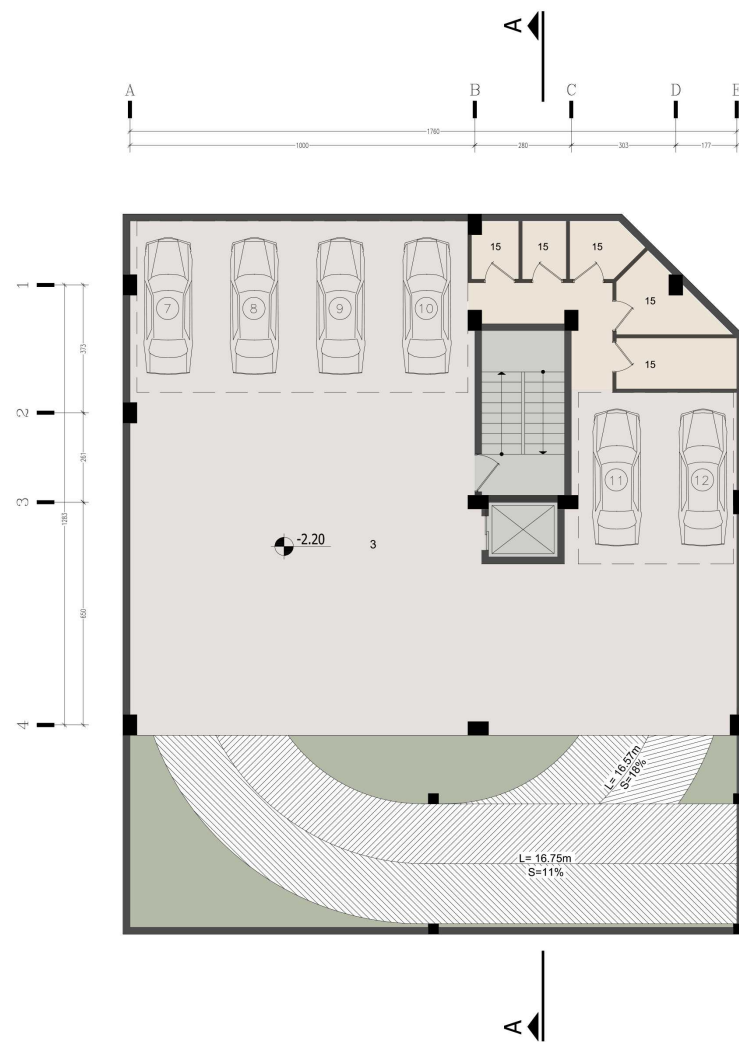
-1 PLAN (FURNITURE)
