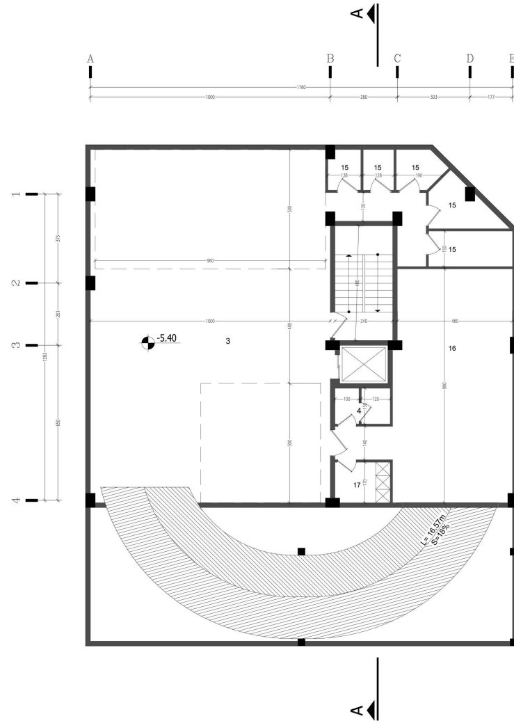
-2 PLAN (DIMENTION)
