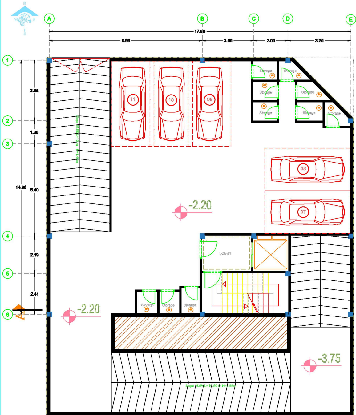
-1 Floor Furniture Plan
