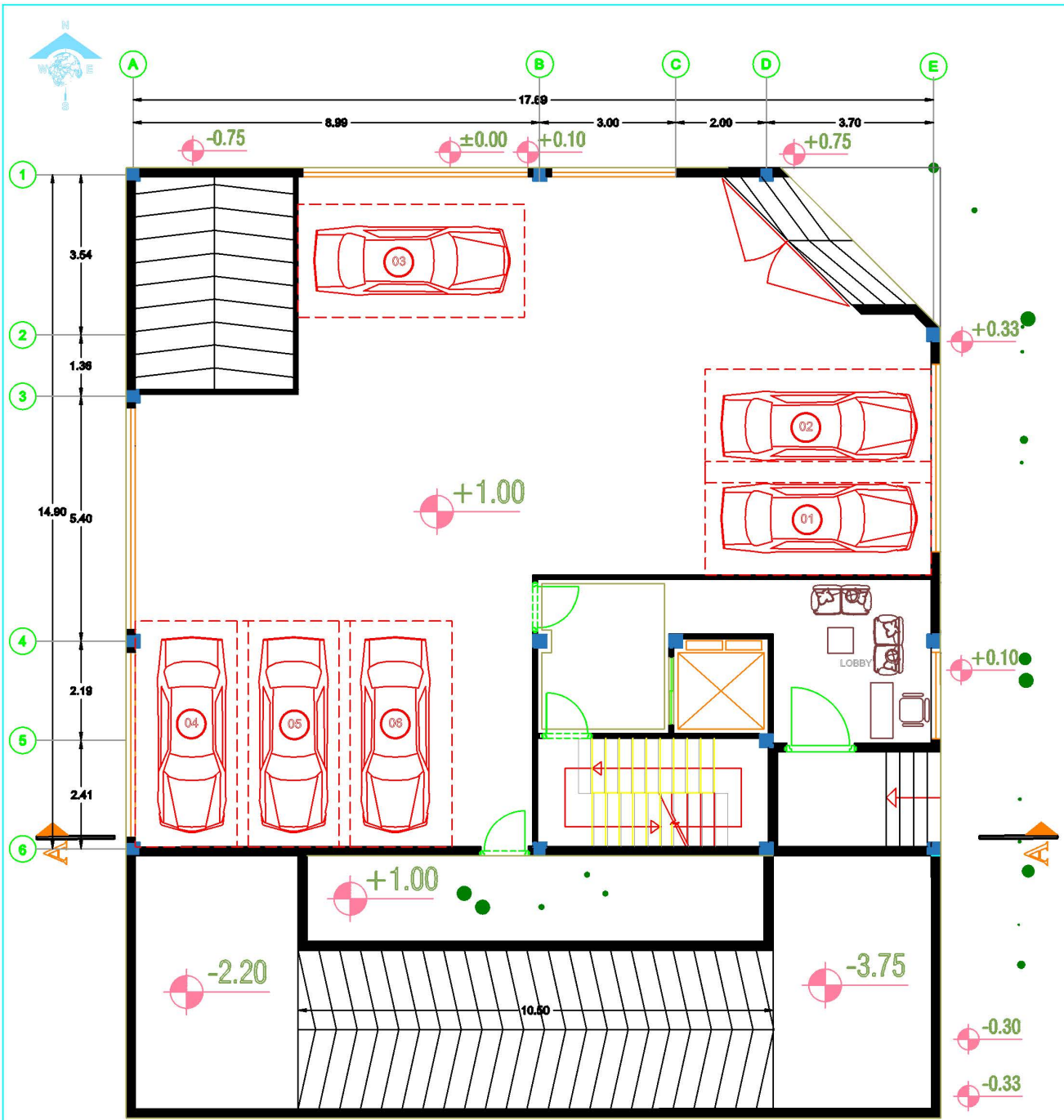
ground Floor Furniture Plan Scale : 1\100
