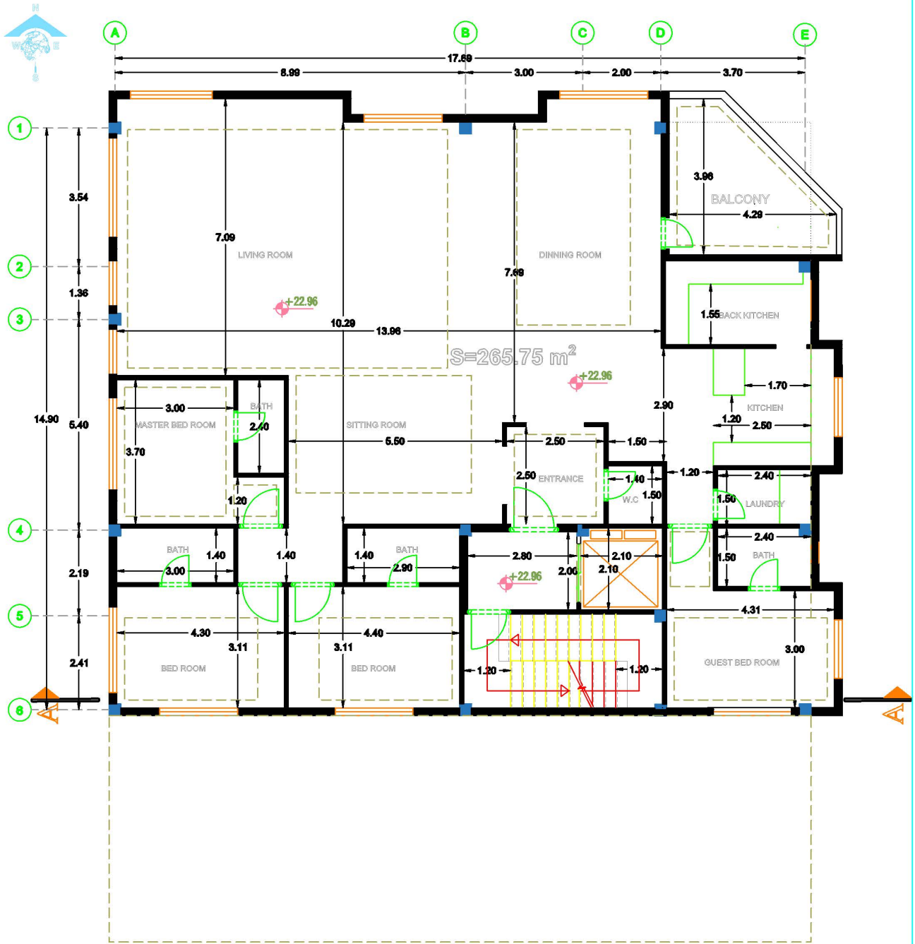
6st Floor Dimension Plan
