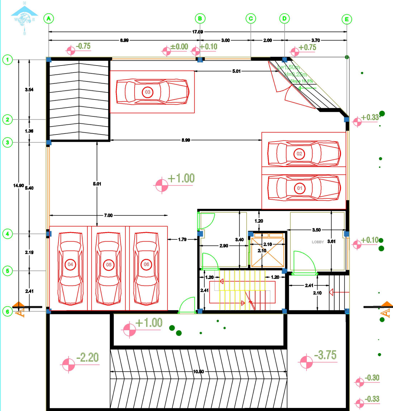
ground Floor Dimension Plan
