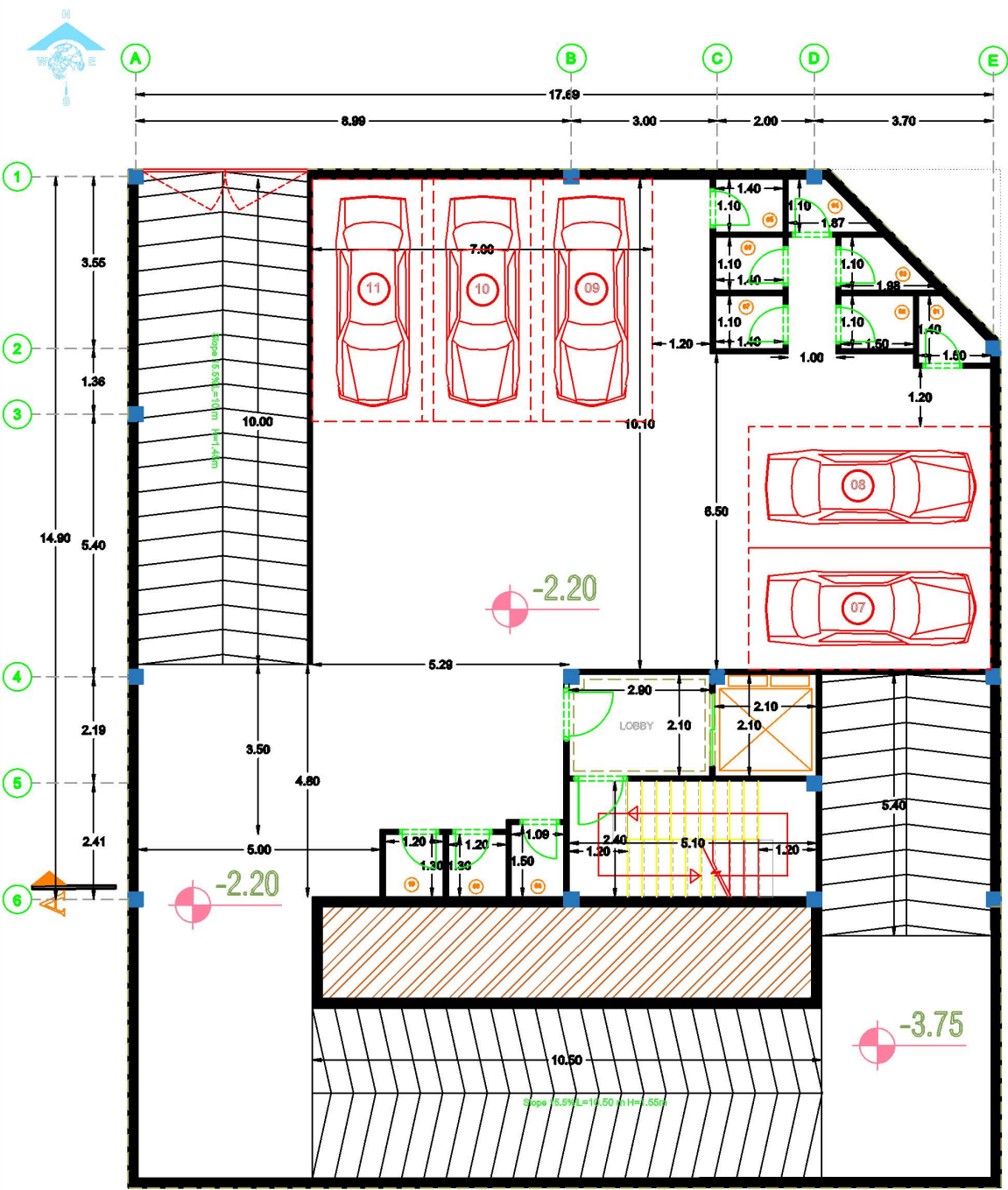
-1 Floor Dimension Plan
