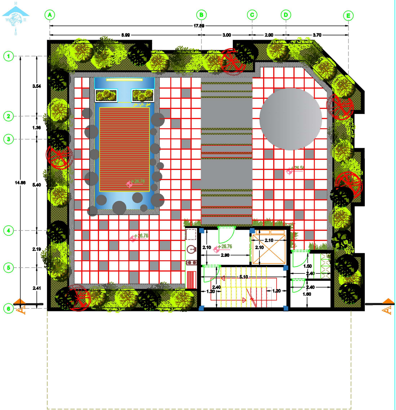
Roof Dimension Plan
