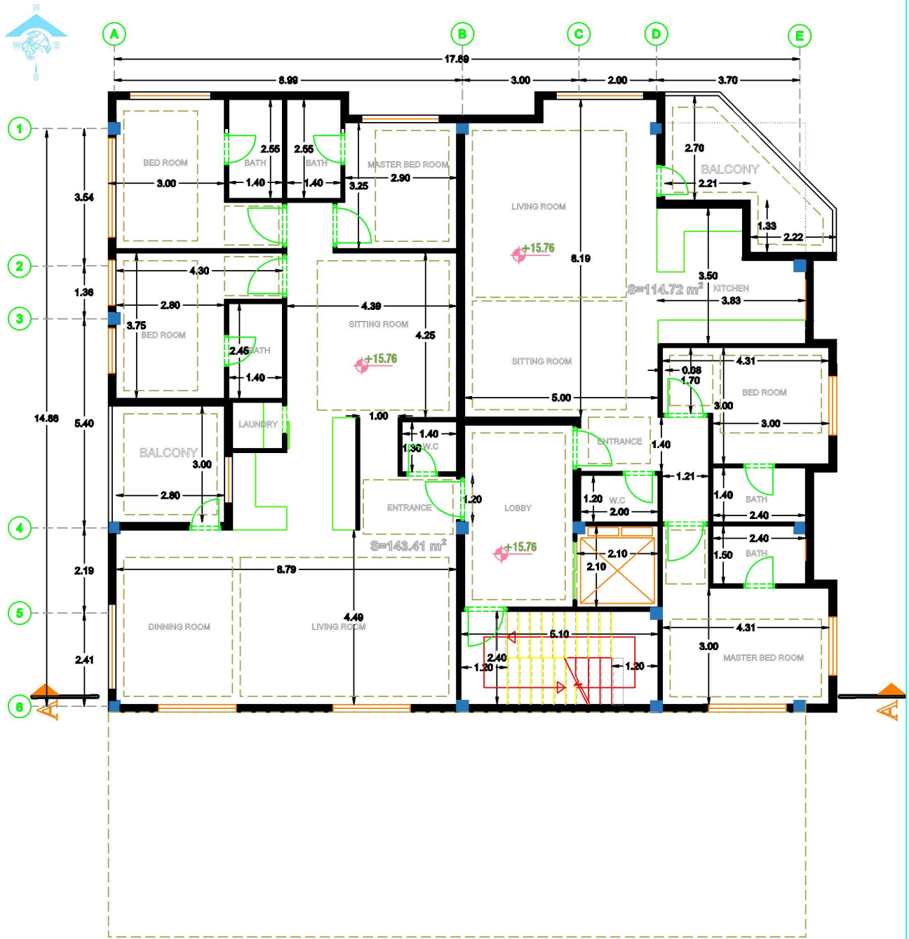
4th Floor Dimension Plan Scale : 1\100
