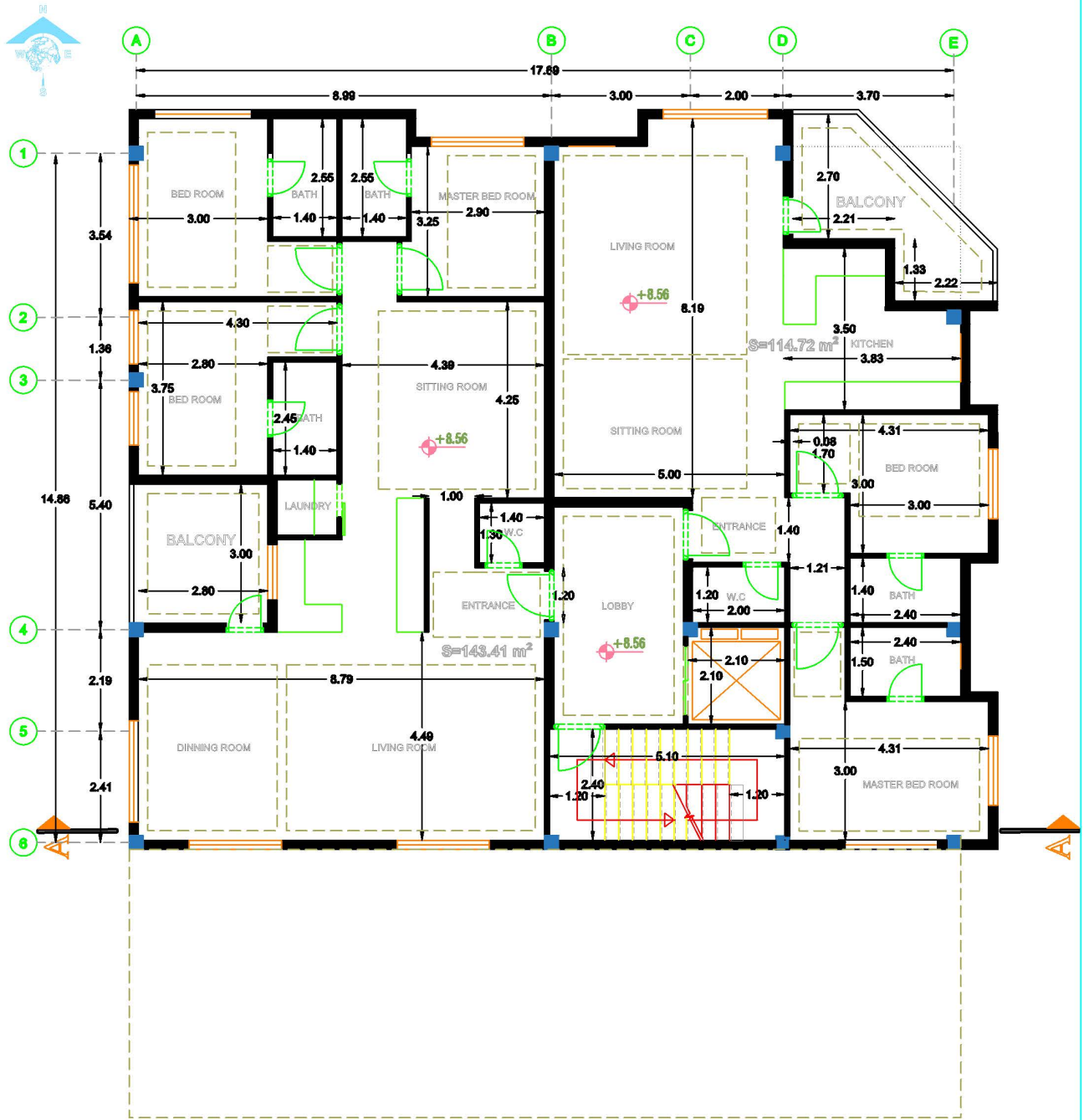
2st Floor Dimension Plan
