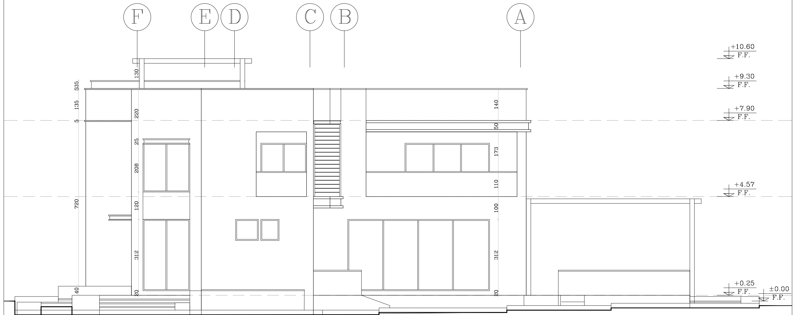
NORTH ELEVATION
