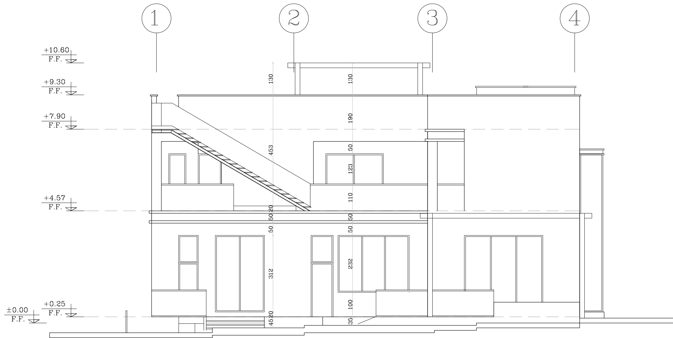
WEST ELEVATION
