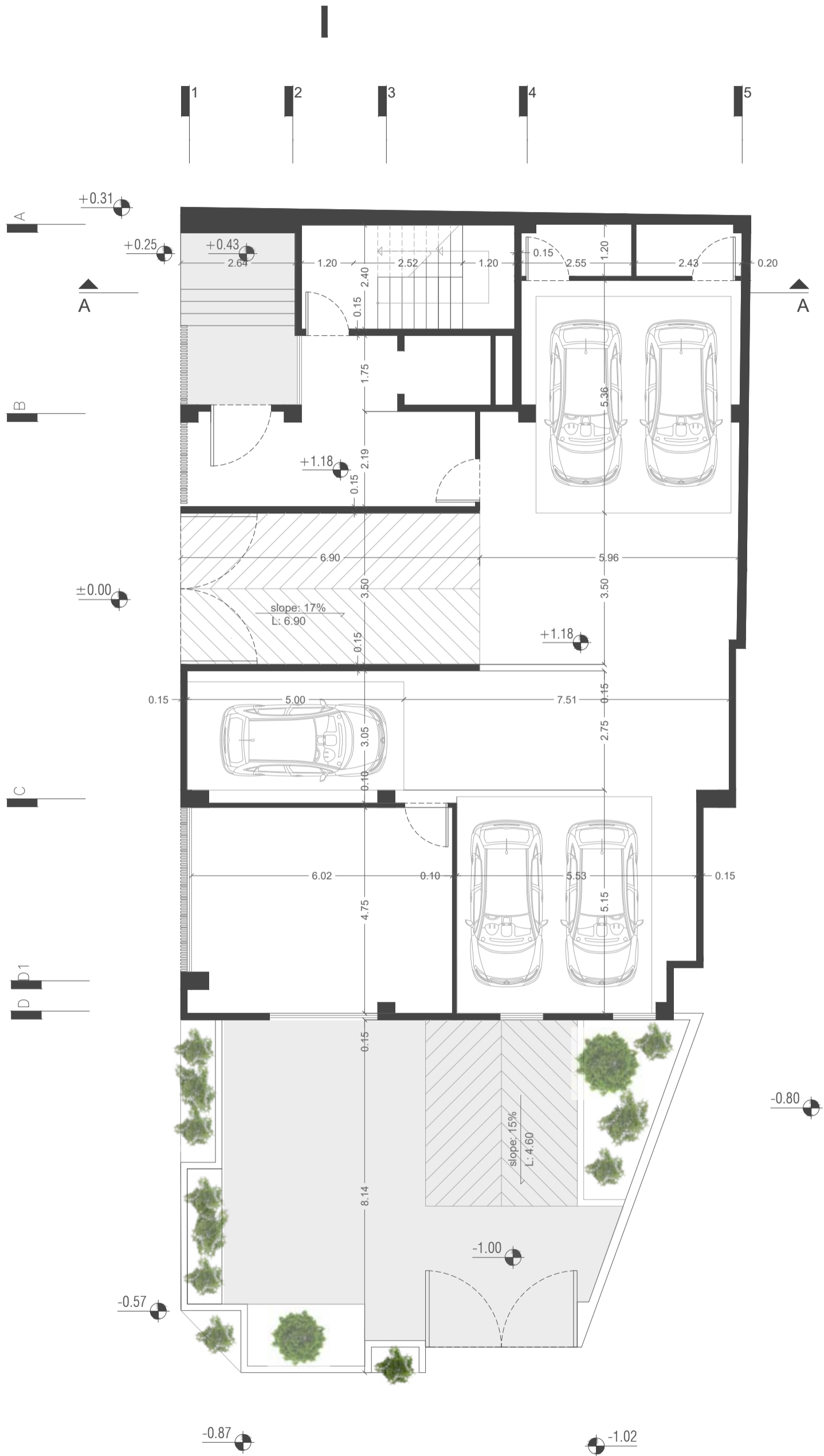
Ground Floor Plan SC : 1/100
