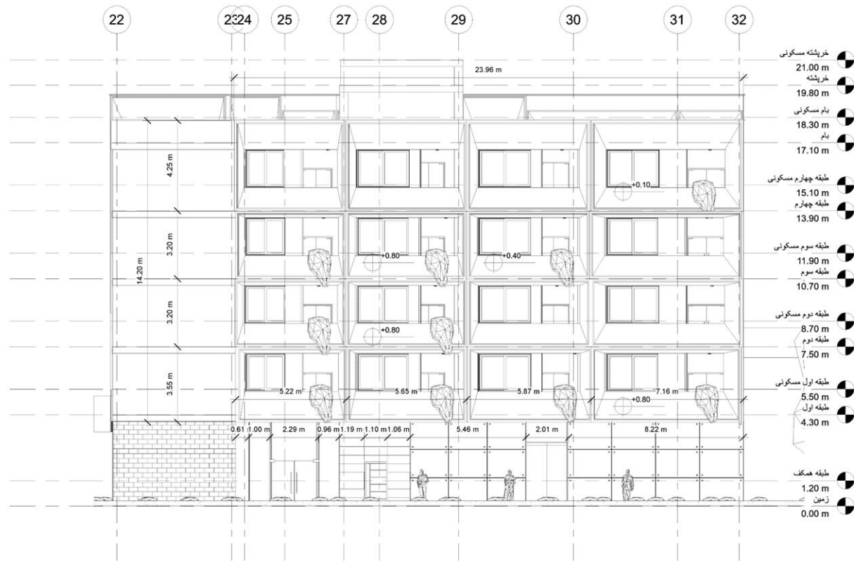
1 South 1 1 : 100
