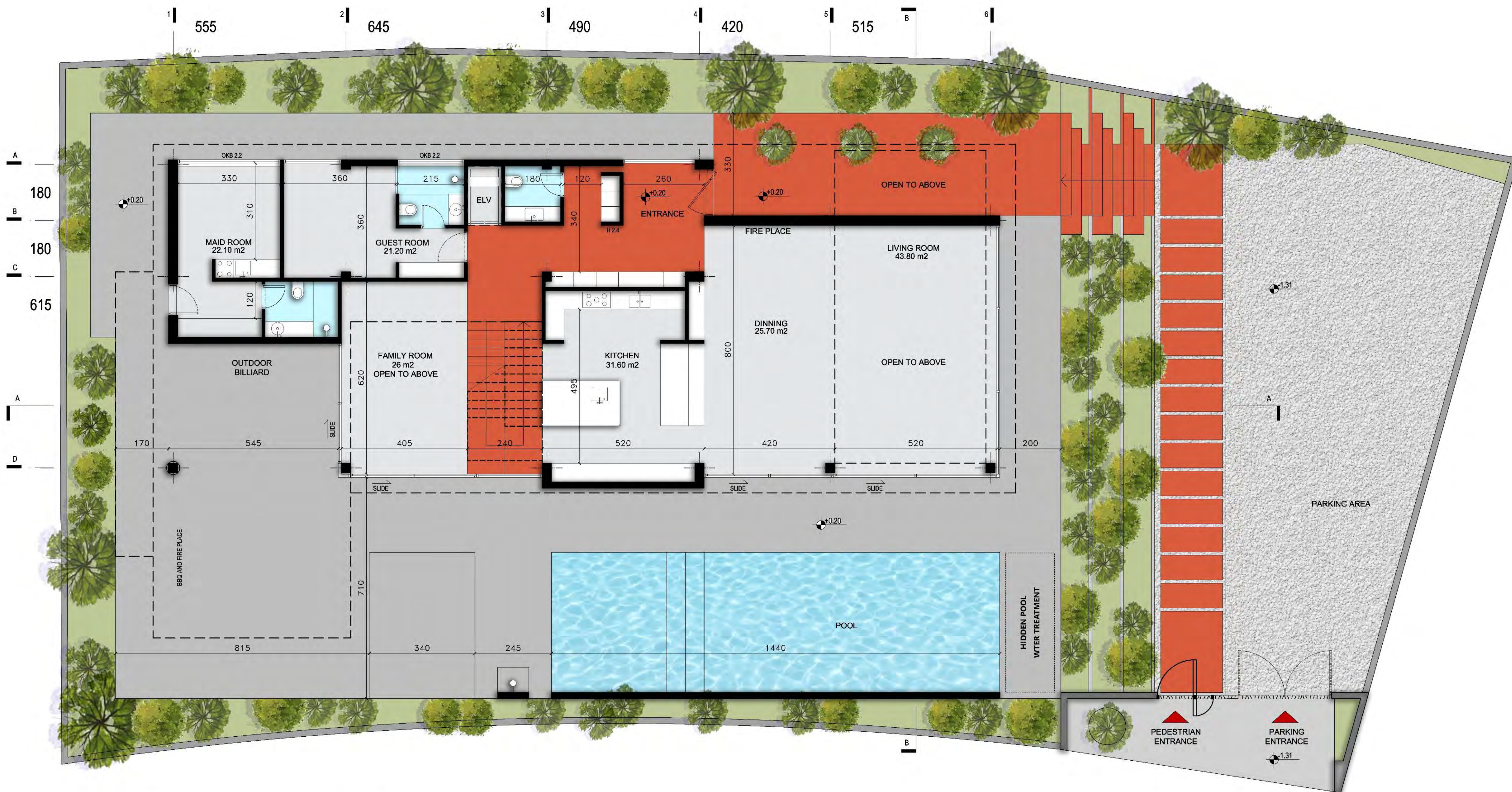
GROUND FLOOR PLAN - DIMENTION
