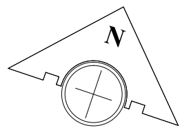
Narenj villa Roof plan SC 1/100
