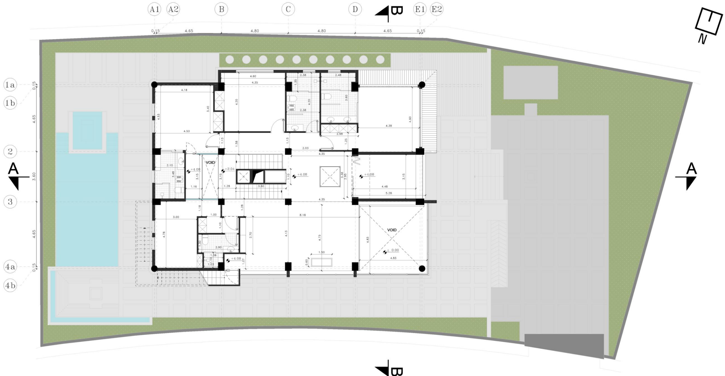
FIRST FLOOR DIMENSION PLAN
