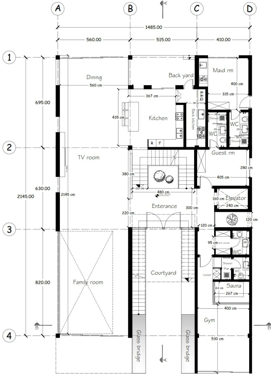
Ground floor Dimension plan
