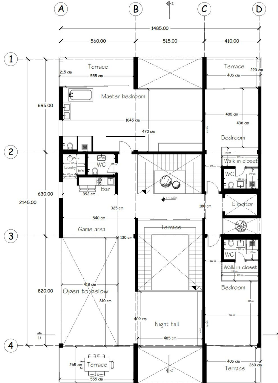
First floor Dimension plan
