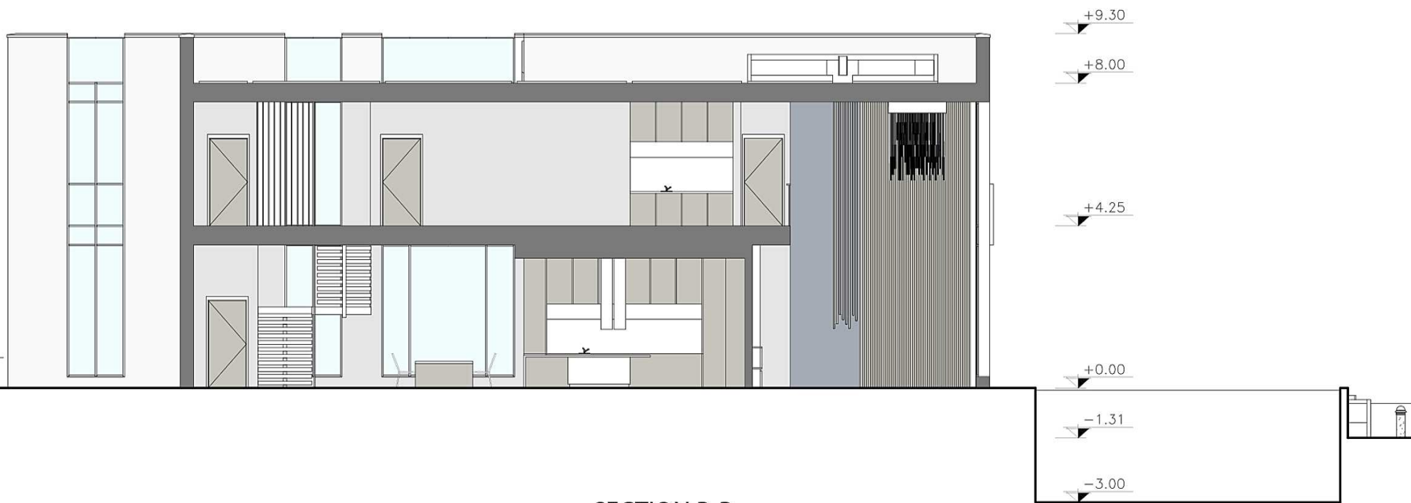
SECTION B-B
