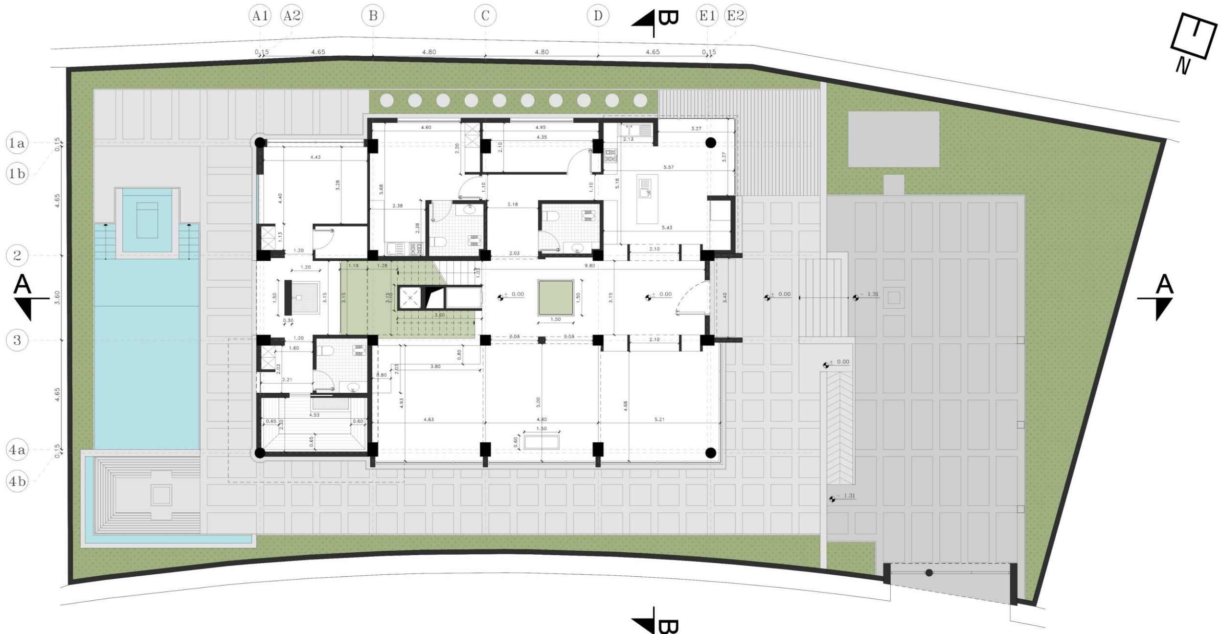
GROUND FLOOR DIMENSION PLAN
