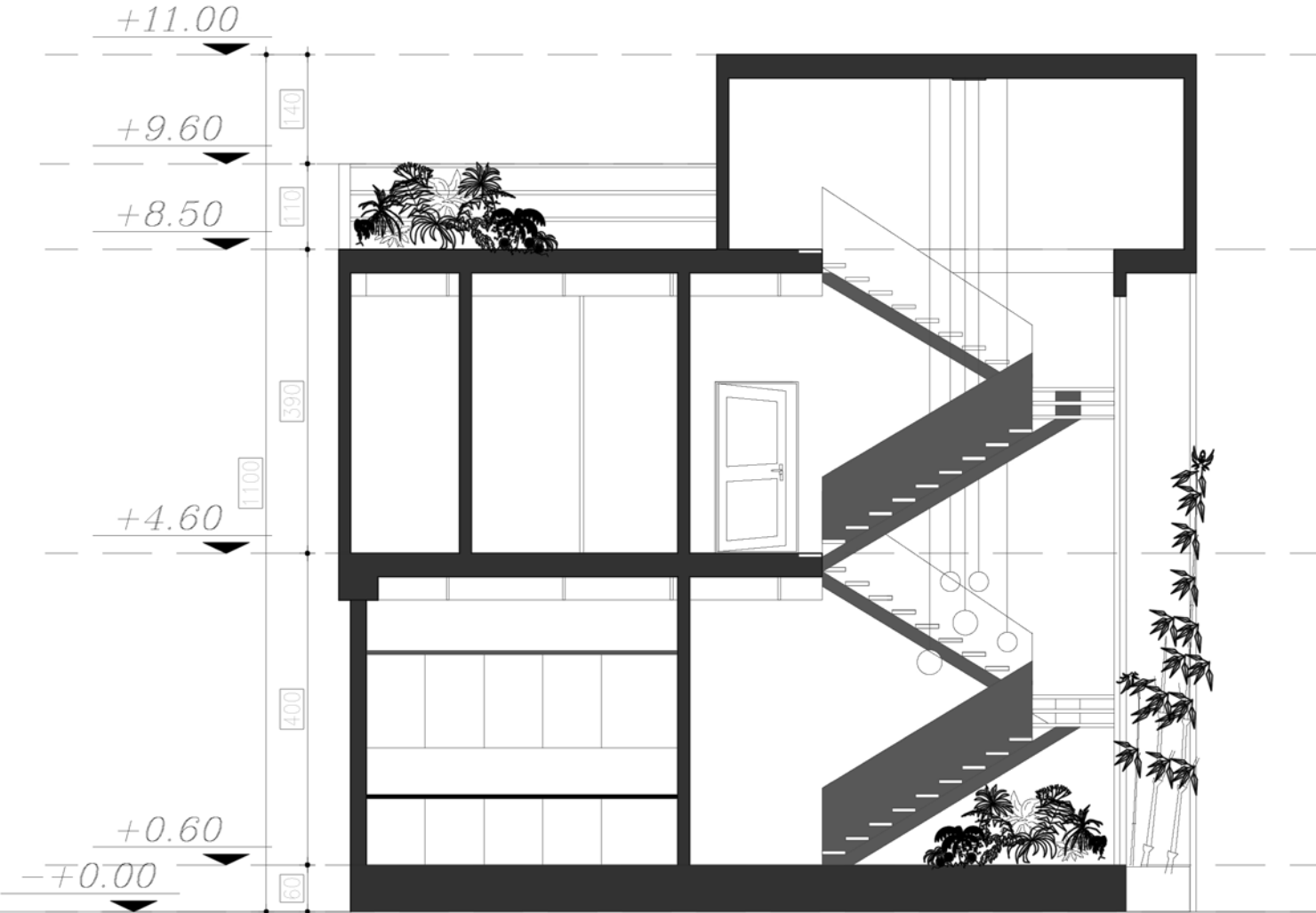
Section BB
