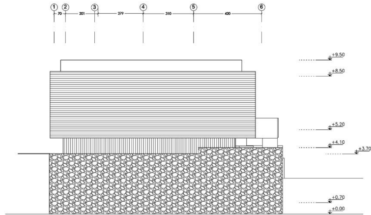
WEST ELEVATION
