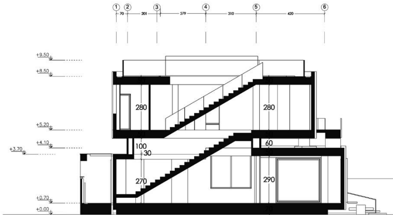
SECTION B-B
