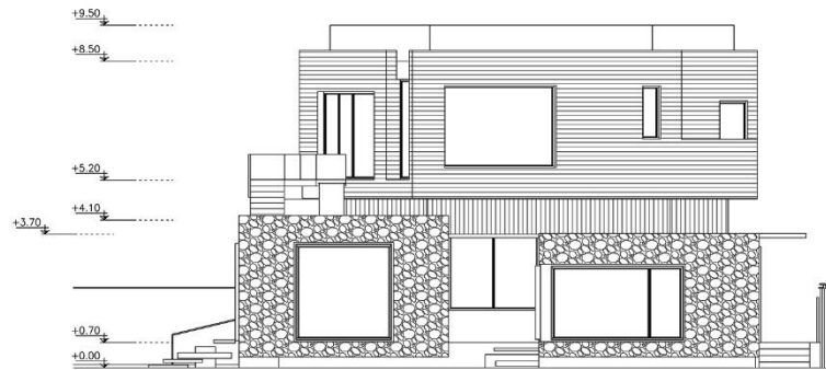
EAST ELEVATION
