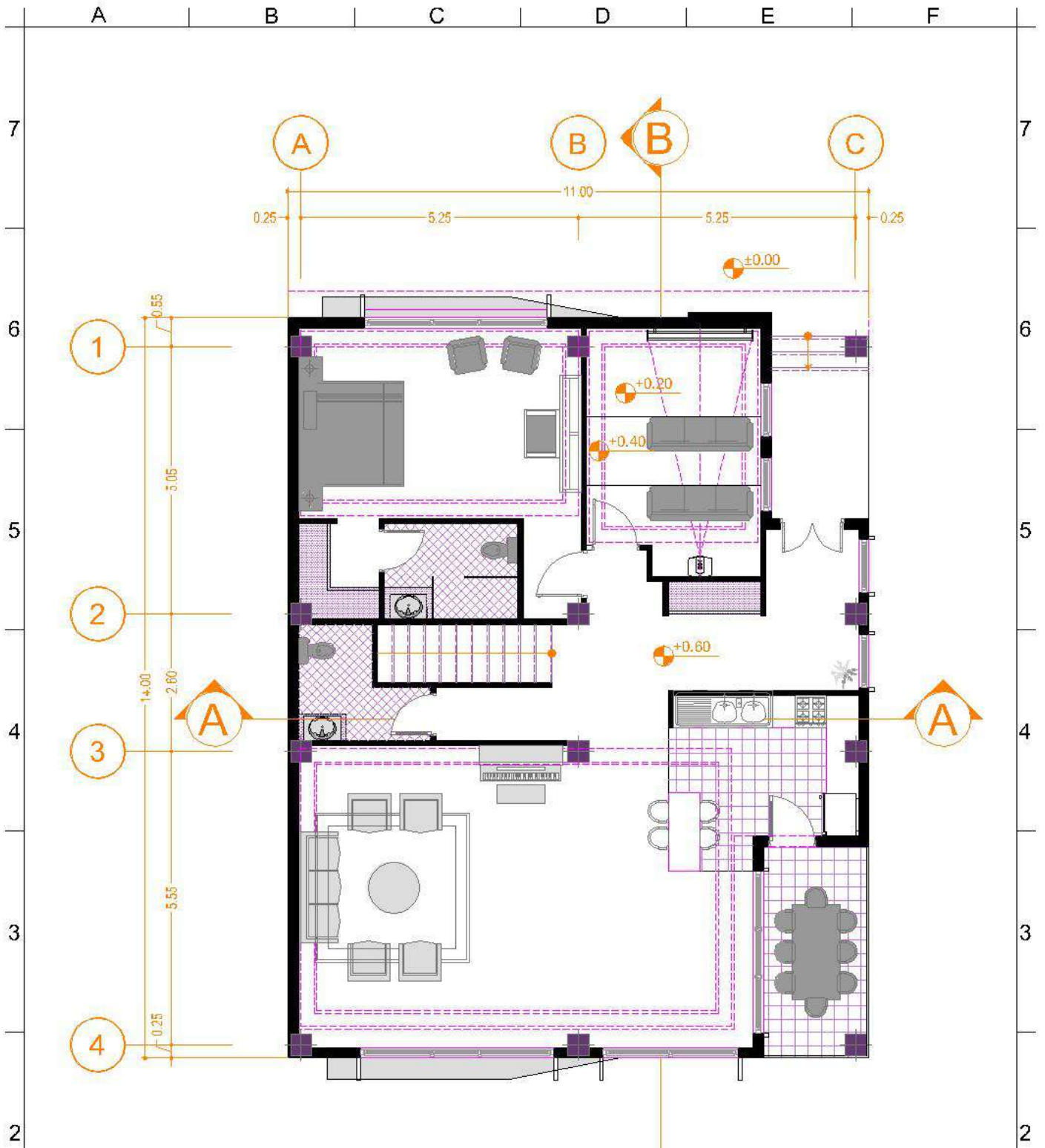
GROUND FLOOR PLAN(fur)
