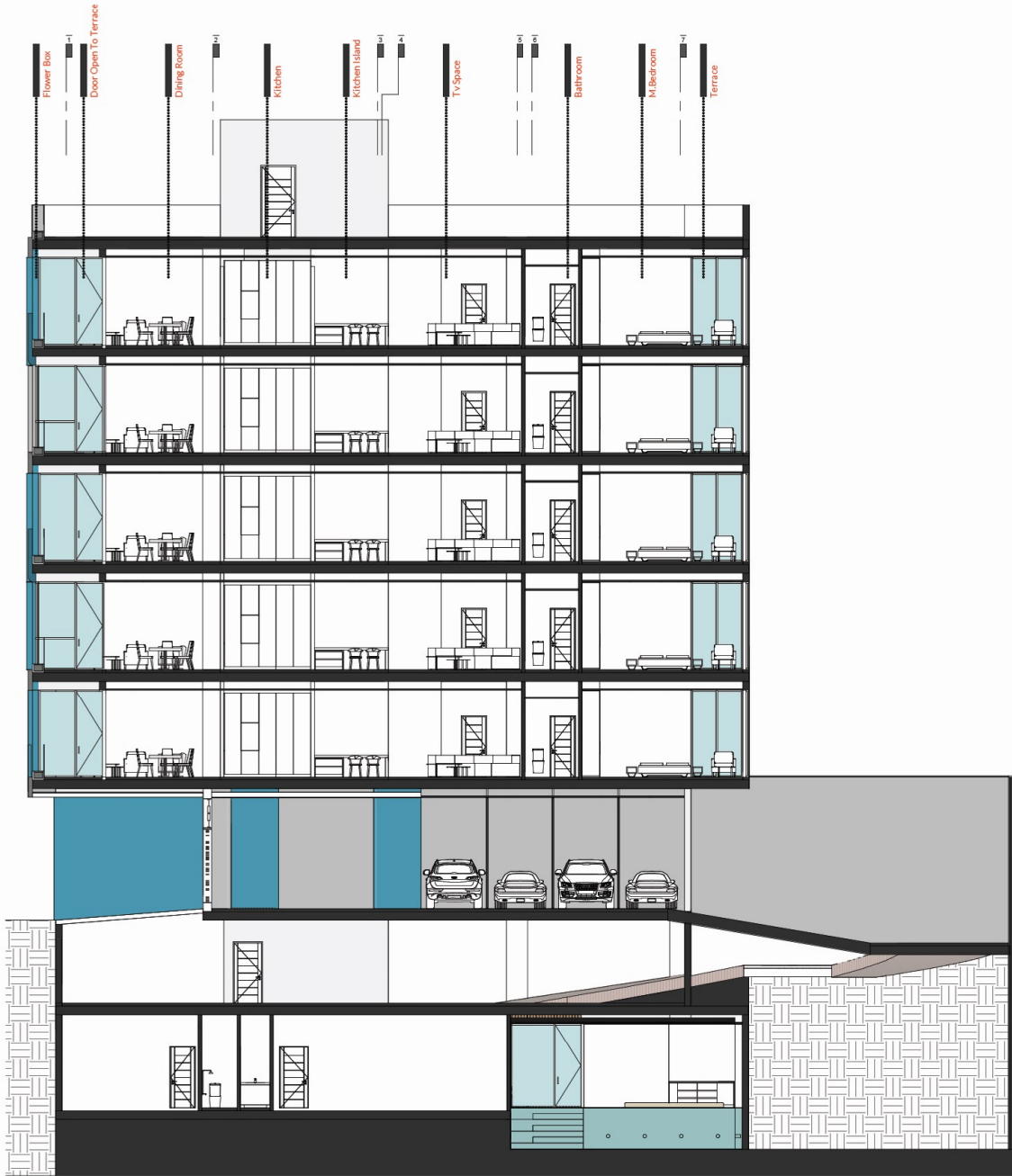
Section B_B 0 1 2 5
