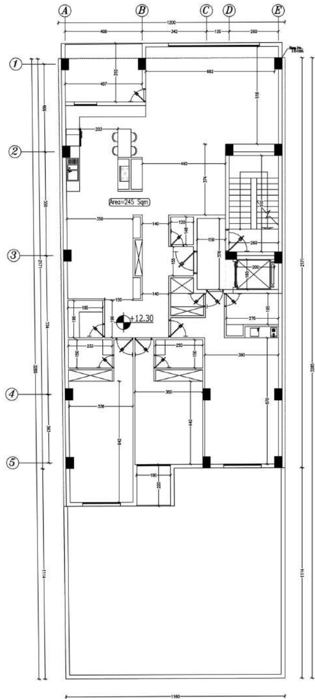
Third Floor Plan Scale=1:100
