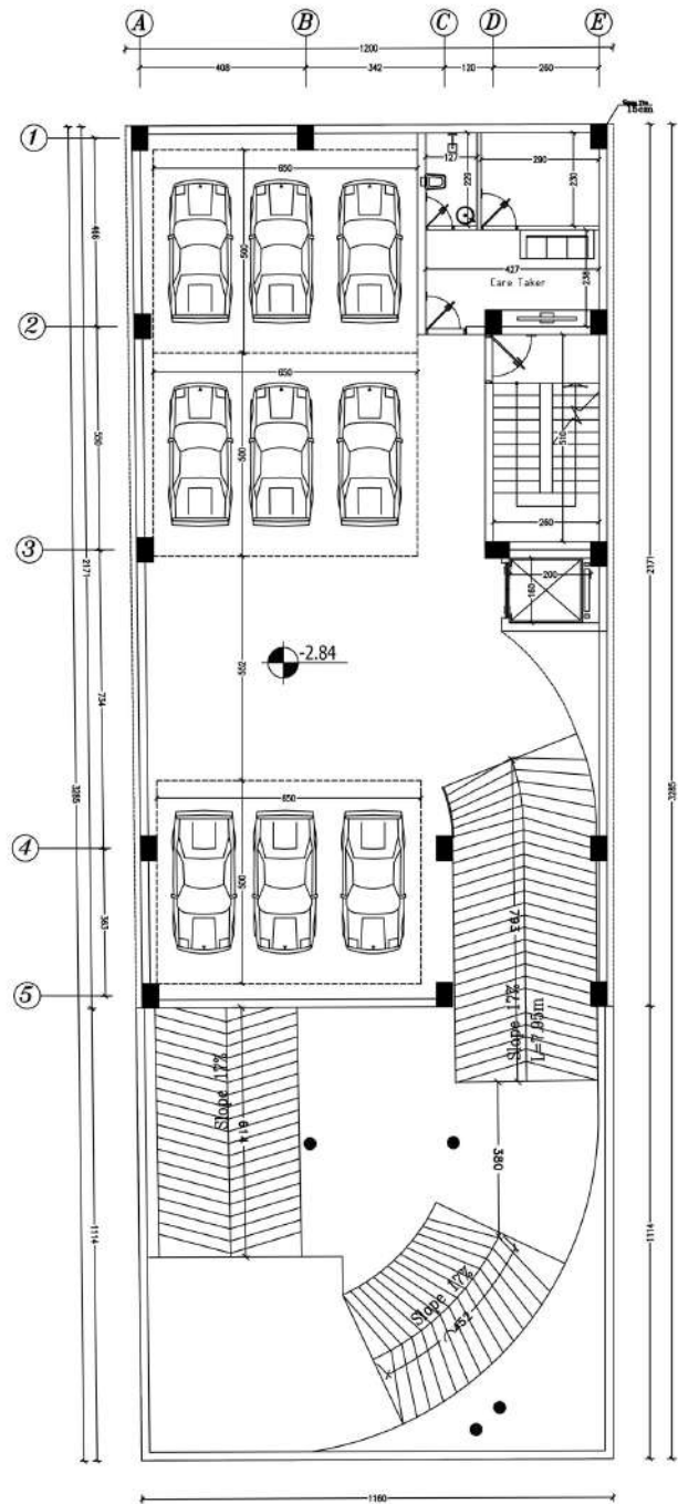
-1 Floor Plan Scale=1:100
