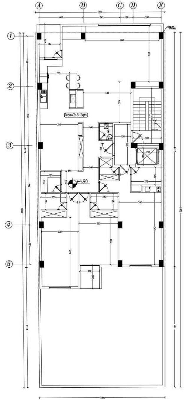
Second Floor Plan Scale=1:100
