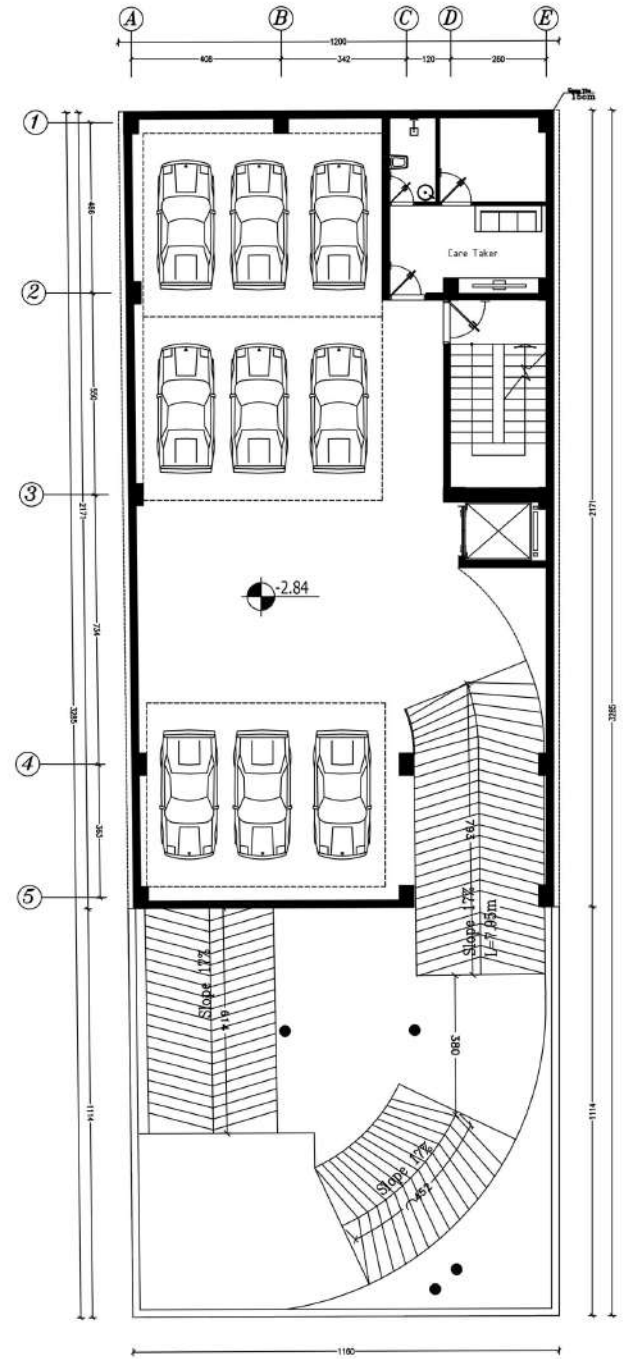
-1 Floor Plan Scale=1:100
