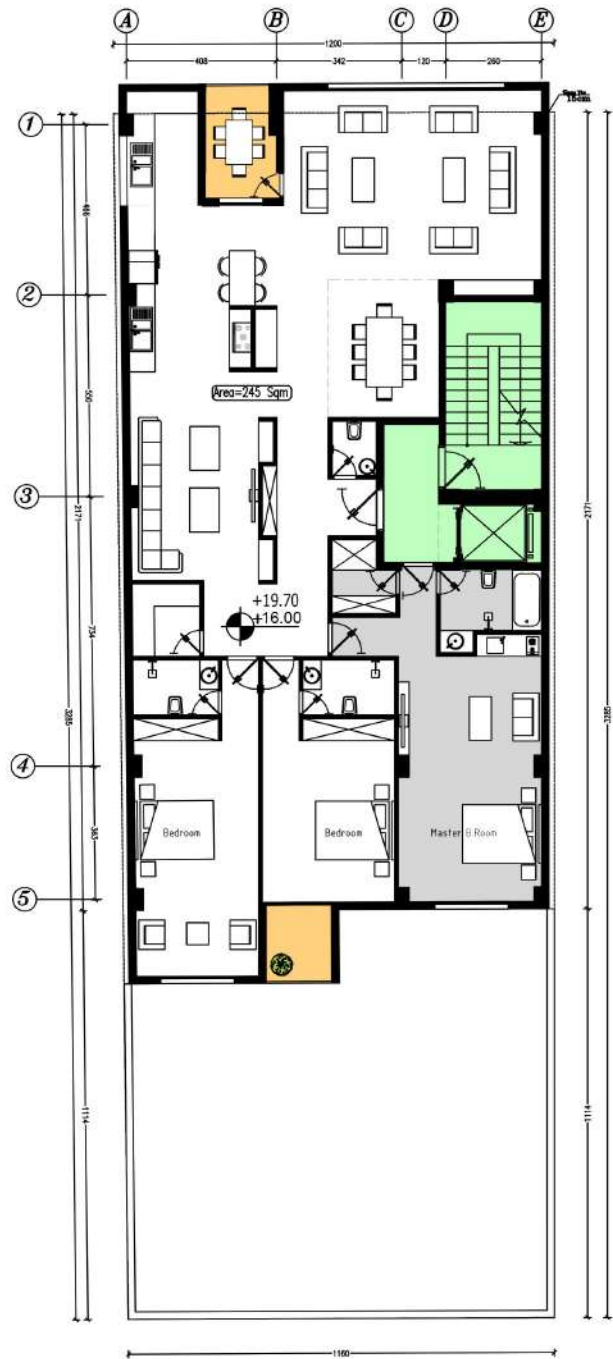
Forth & Fifth Floor Plan Scale=1:100
