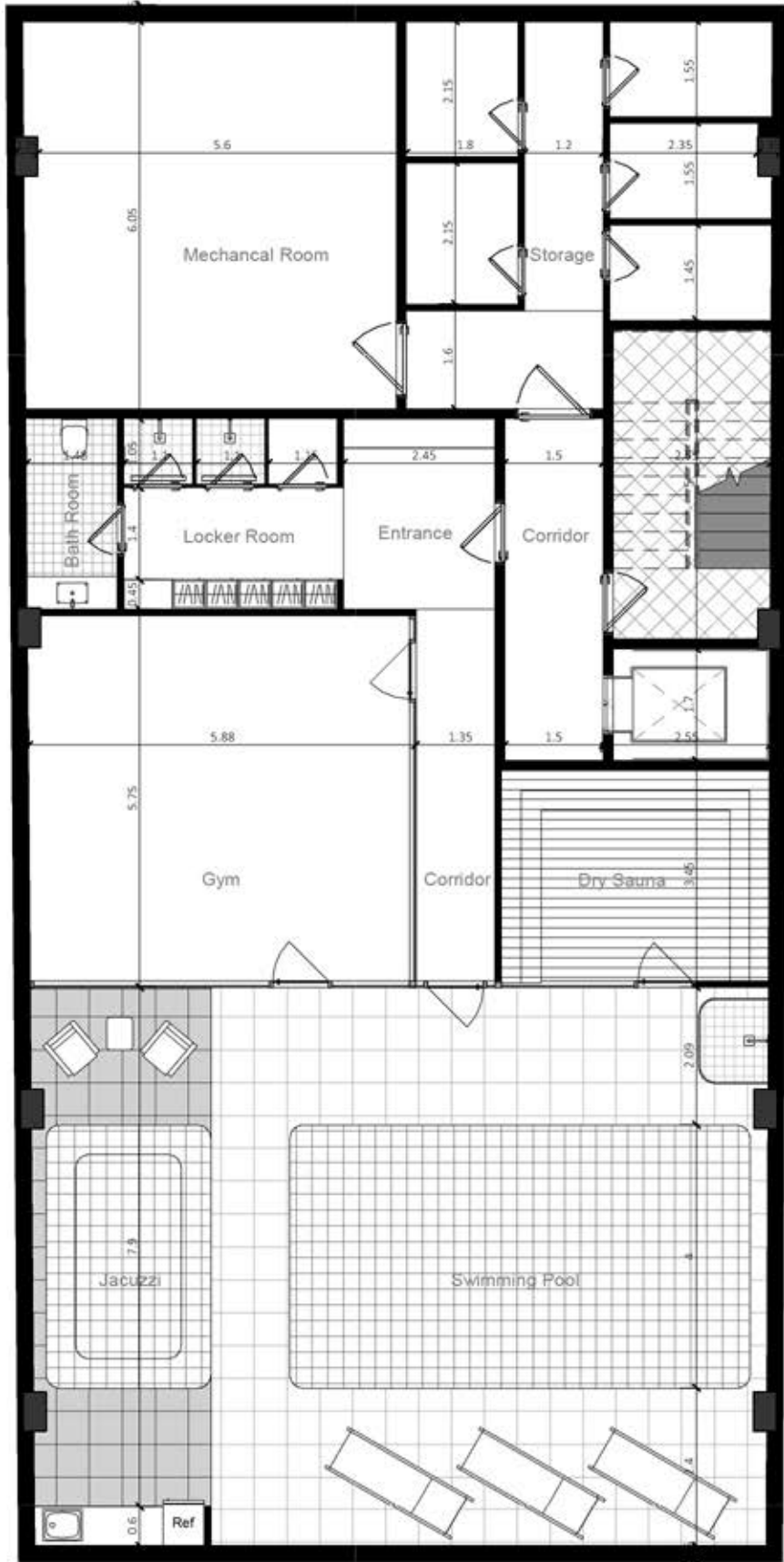
Basement 2 Plan
