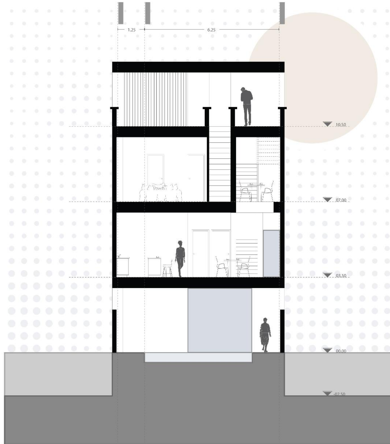
Section B-B
