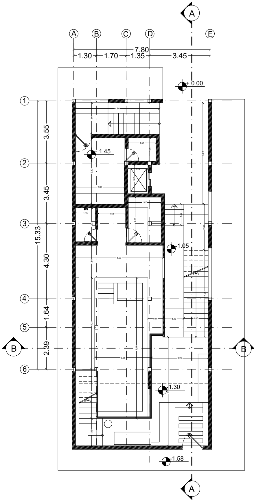
ground plan
