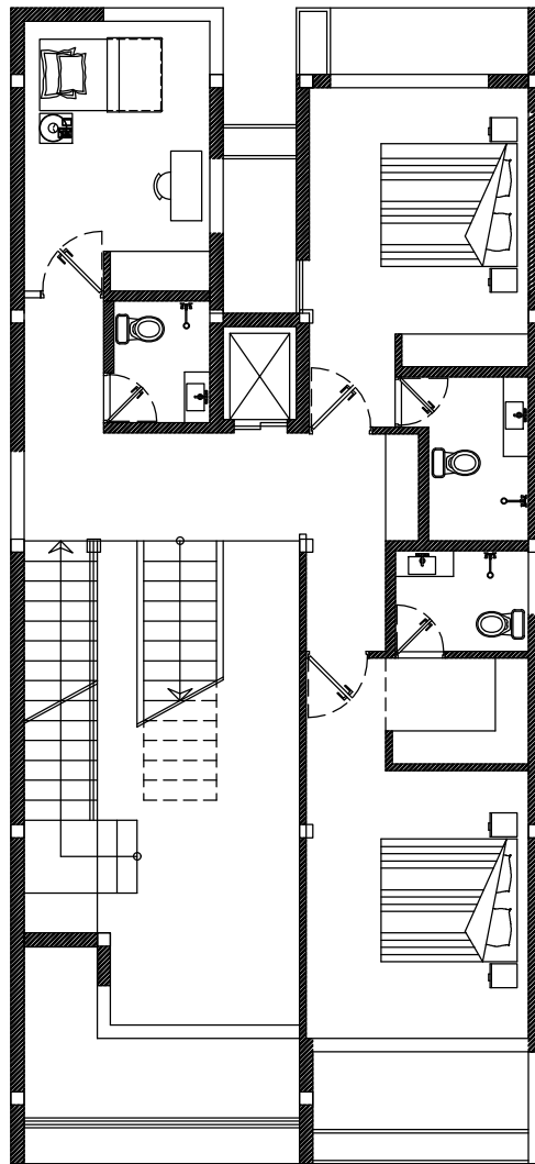
second plan
