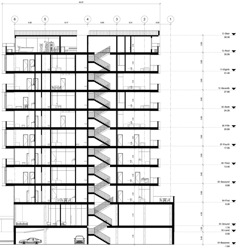
Section AA-Sc: 1.100
