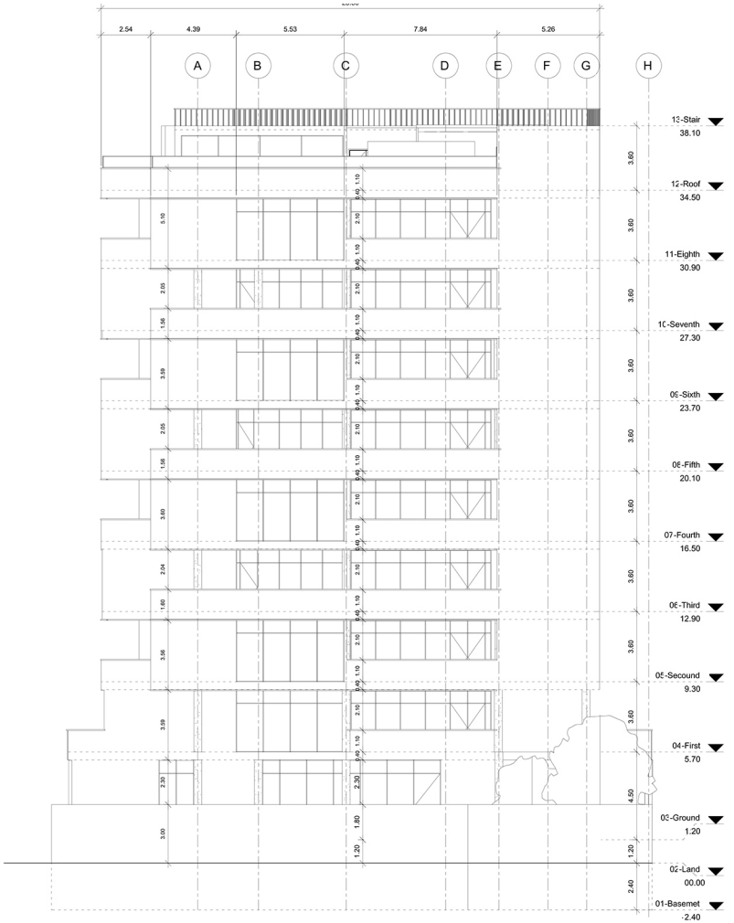
South Facade-Sc: 1.100
