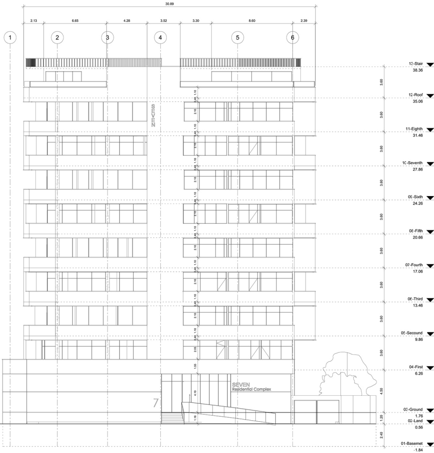
West Facade-Sc: 1.100
