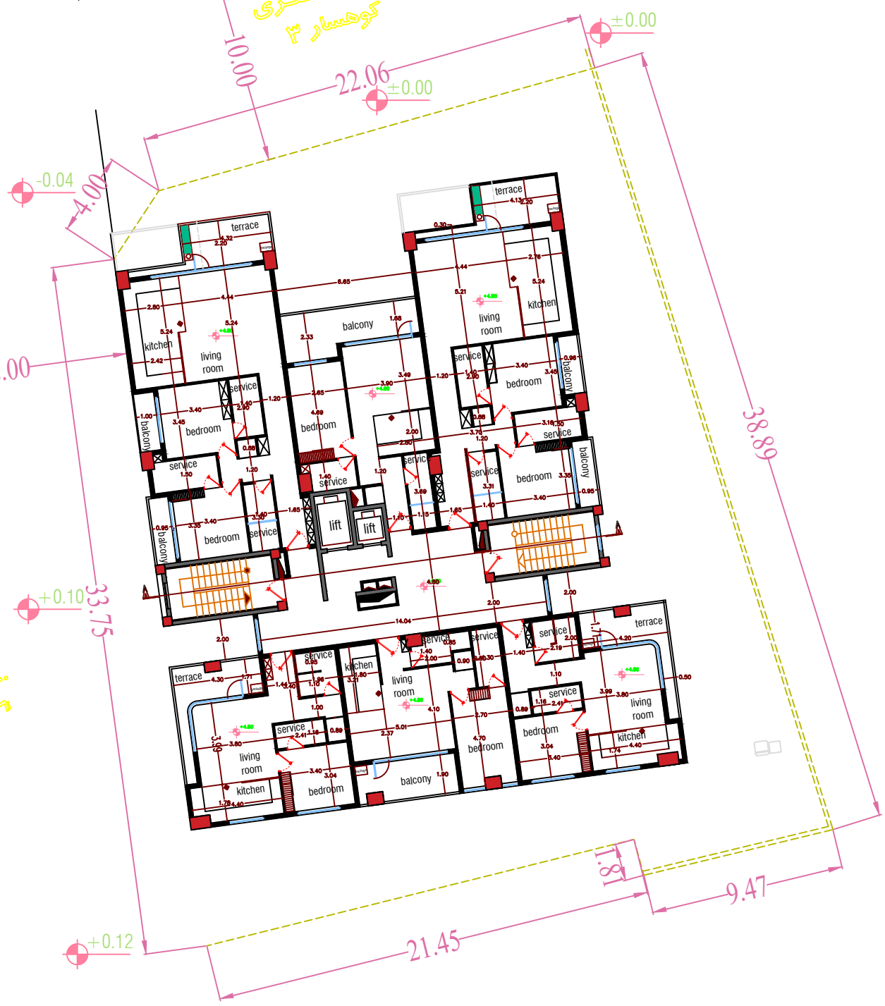
Measurement plan of 1st to 4th floor
