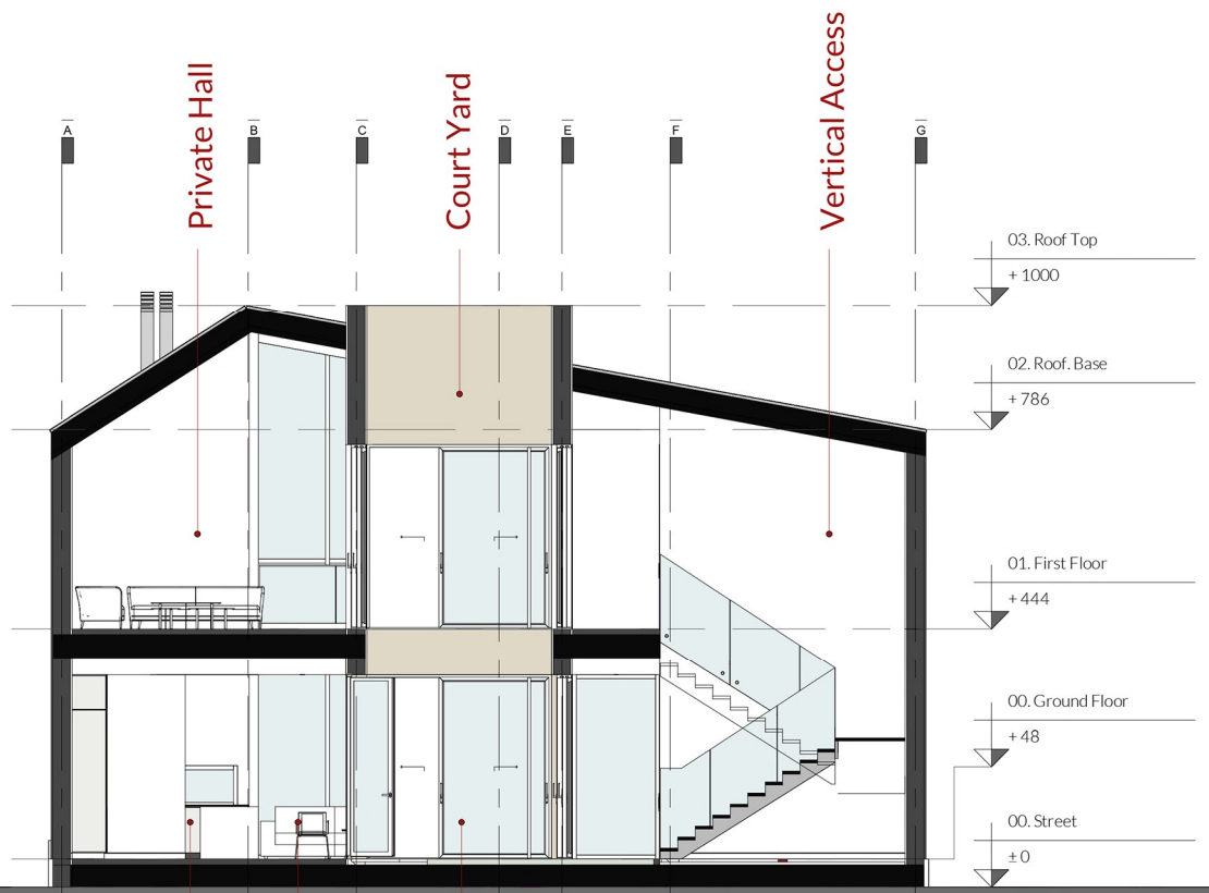
Section A_A 0 1 2 5
