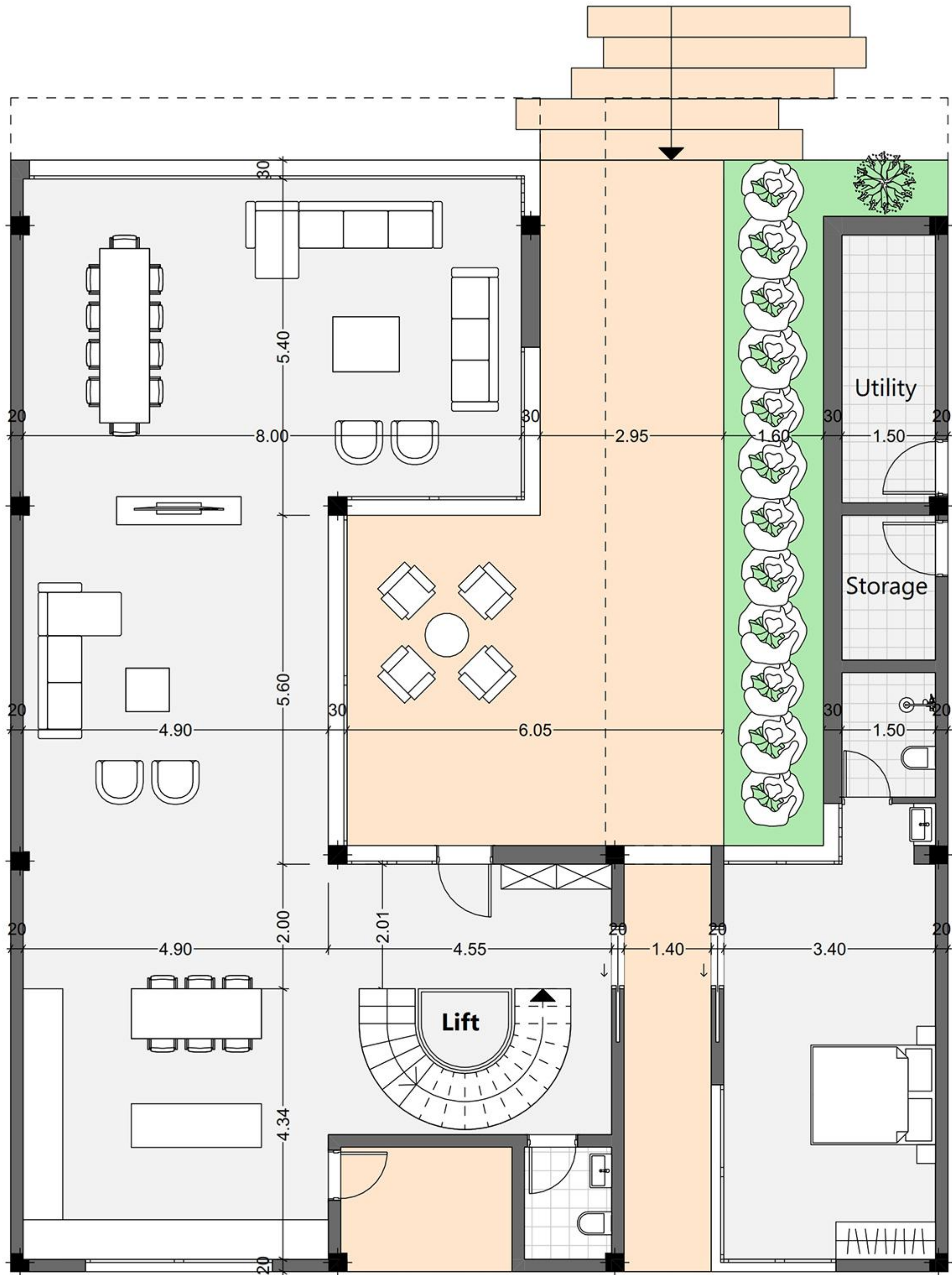
Ground Floor
