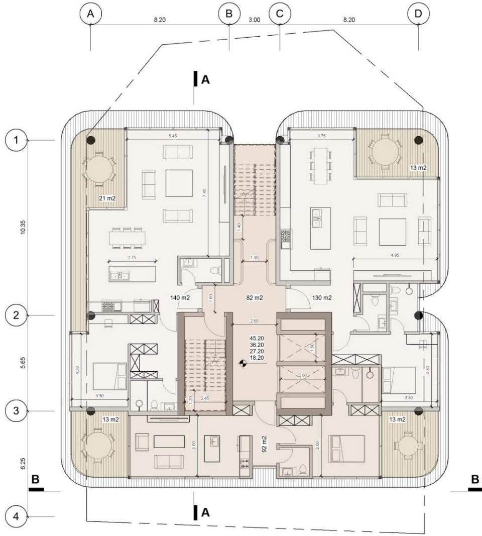
LEVEL 2,4,6,8 FLOOR PLAN
