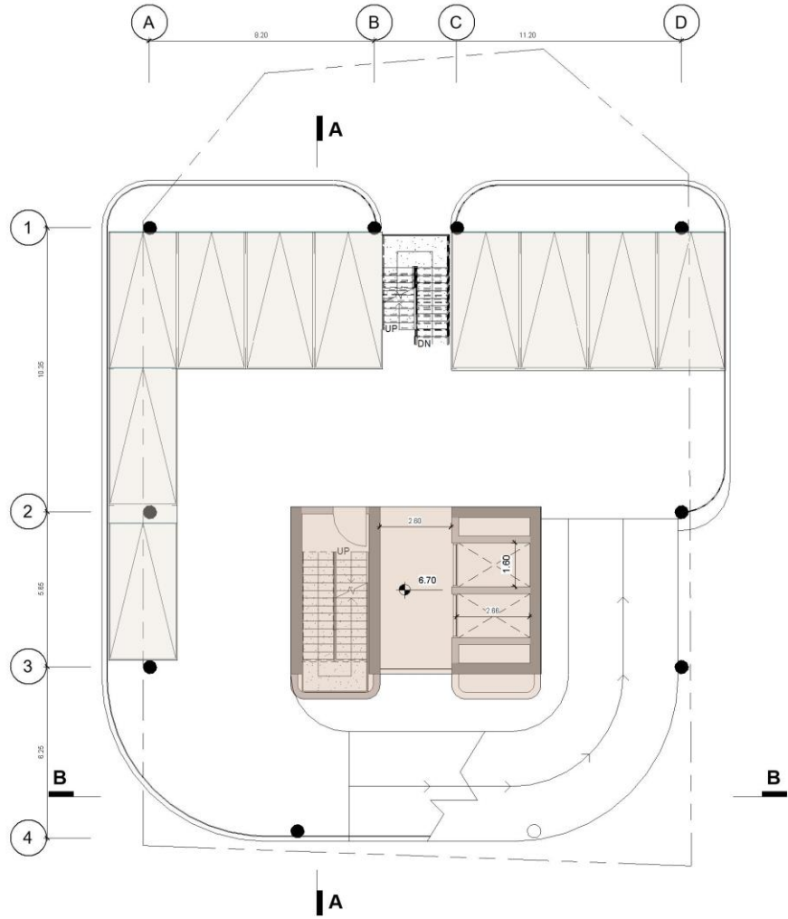
LEVEL P1 FLOOR PLAN 32 PARKING PROVIDED
