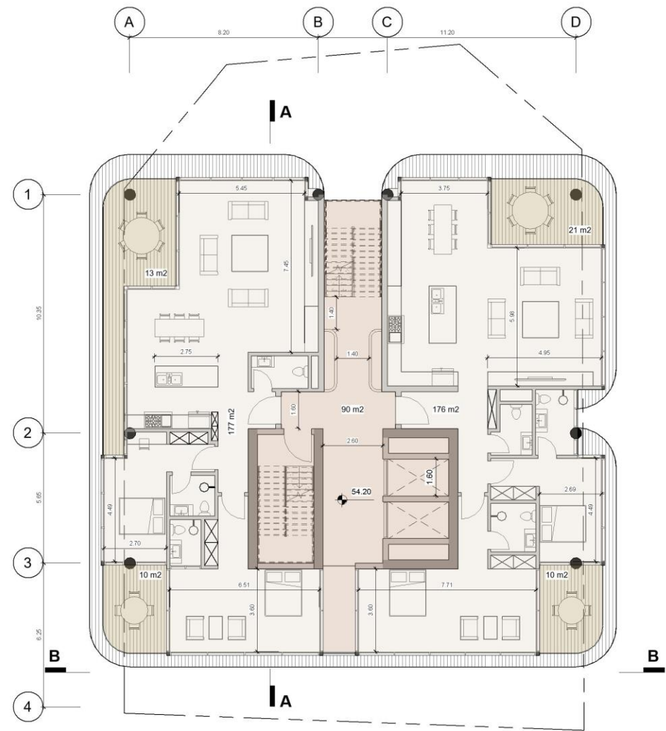
LEVEL 10 FLOOR PLAN
