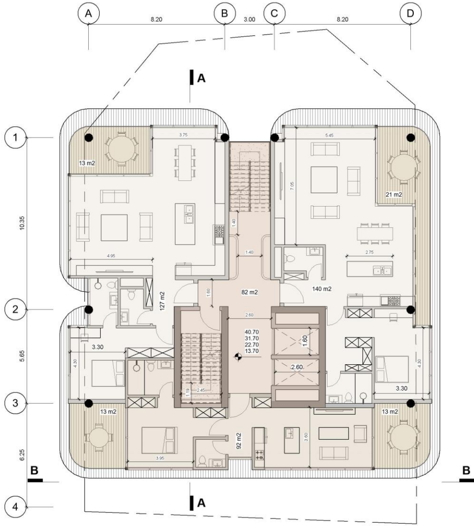
LEVEL 1,3,5,7 FLOOR PLAN
