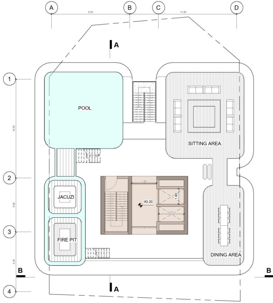
ROOF FLOOR PLAN
