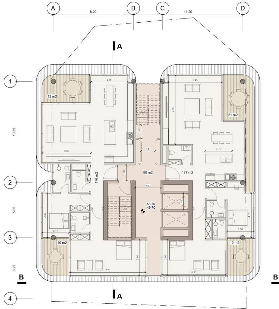
LEVEL 9,11 FLOOR PLAN
