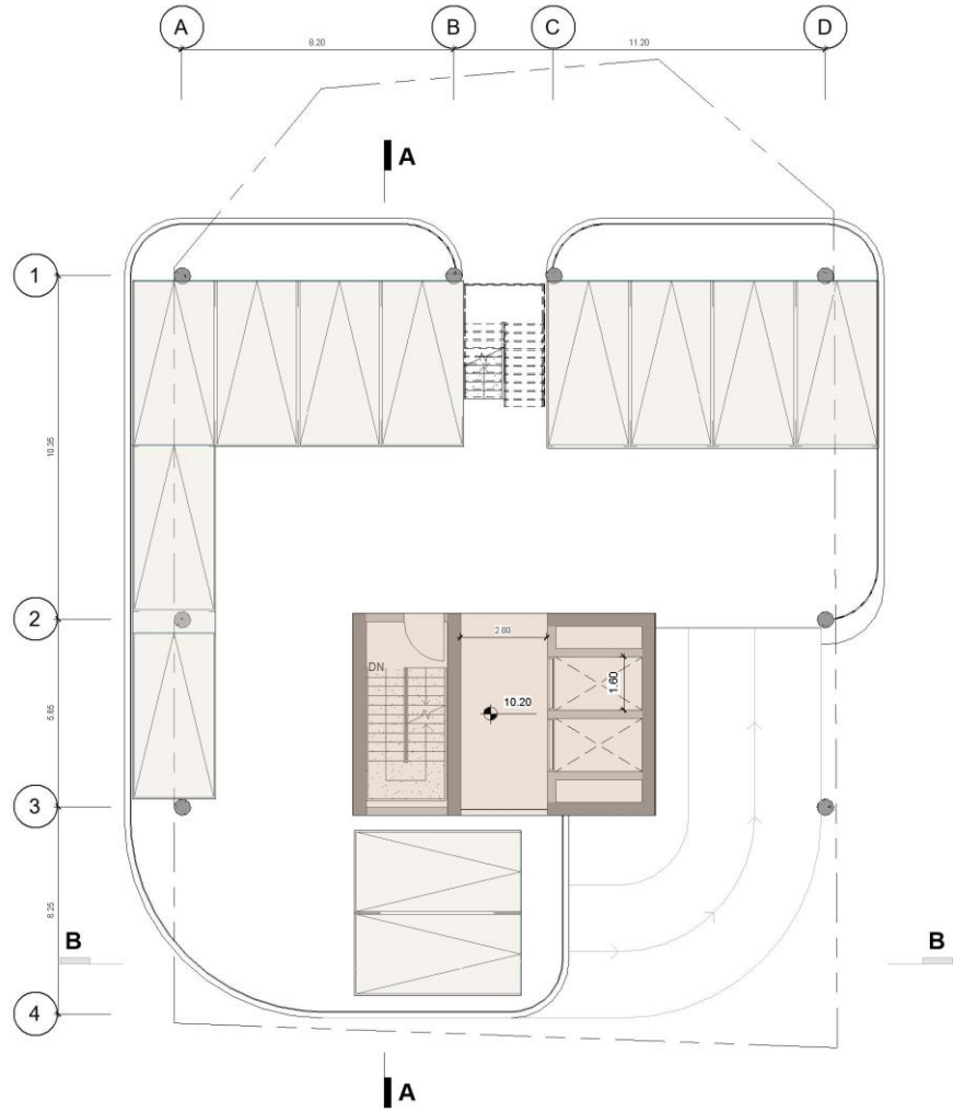
LEVEL P2 FLOOR PLAN 32 PARKING PROVIDED
