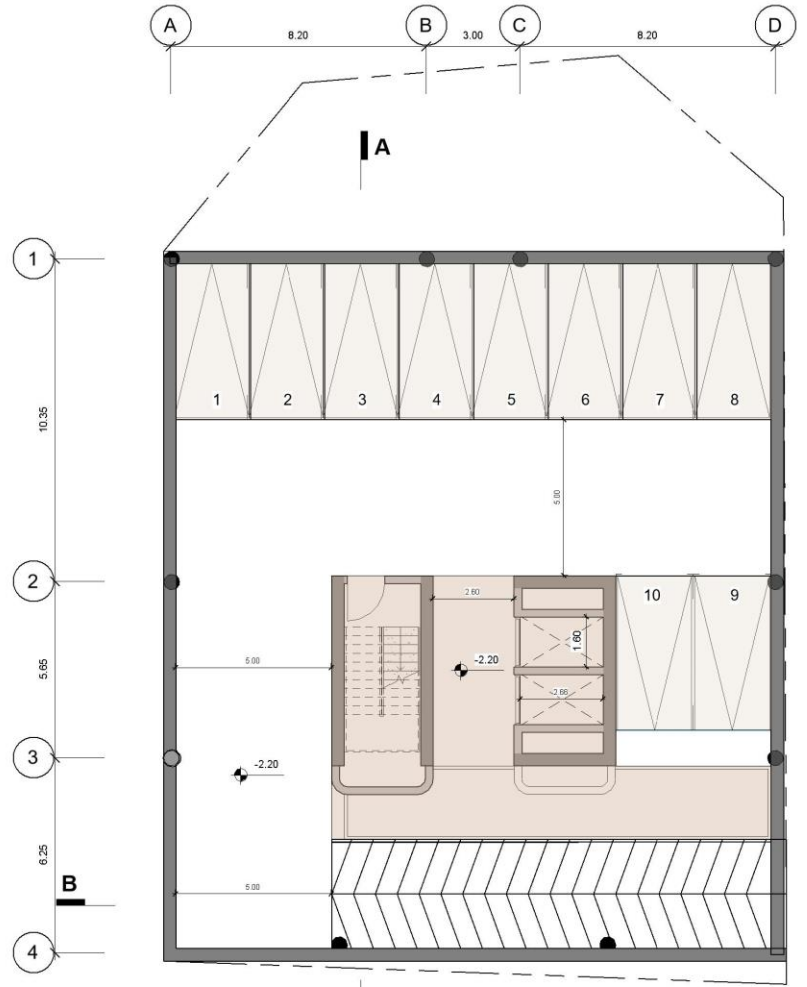
A LEVEL -1 FLOOR PLAN 32 PARKING PROVIDED
