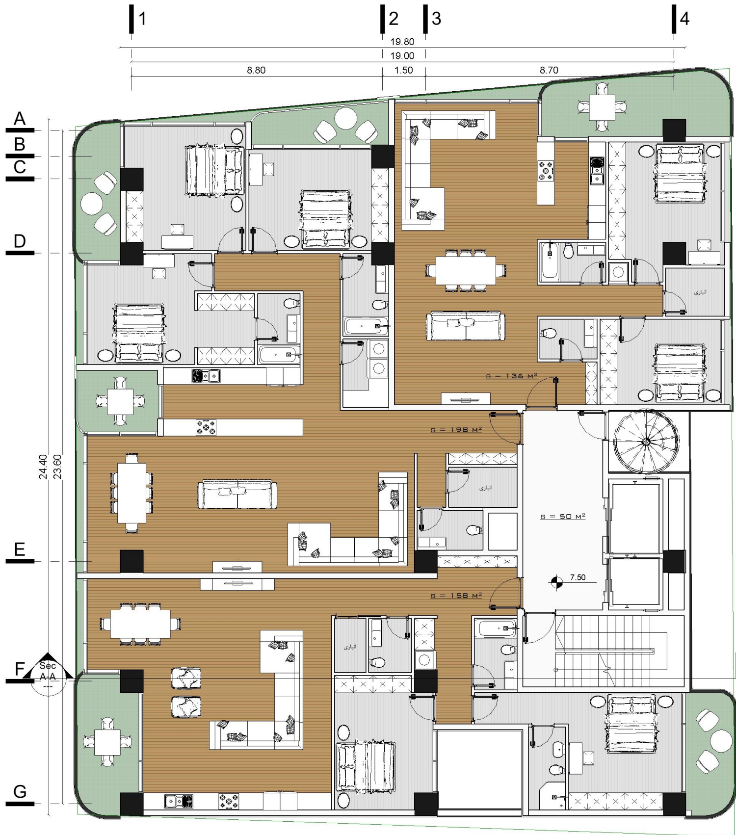
+1,2,4,7 FLOOR FURNITURE PLAN TOTAL AREA = 545 M 2
