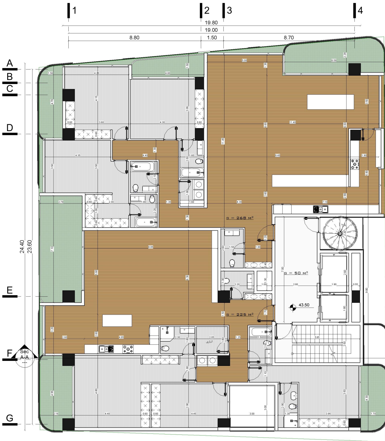
+9,10 FLOOR DIMENTION PLAN TOTAL AREA = 545 M 2
