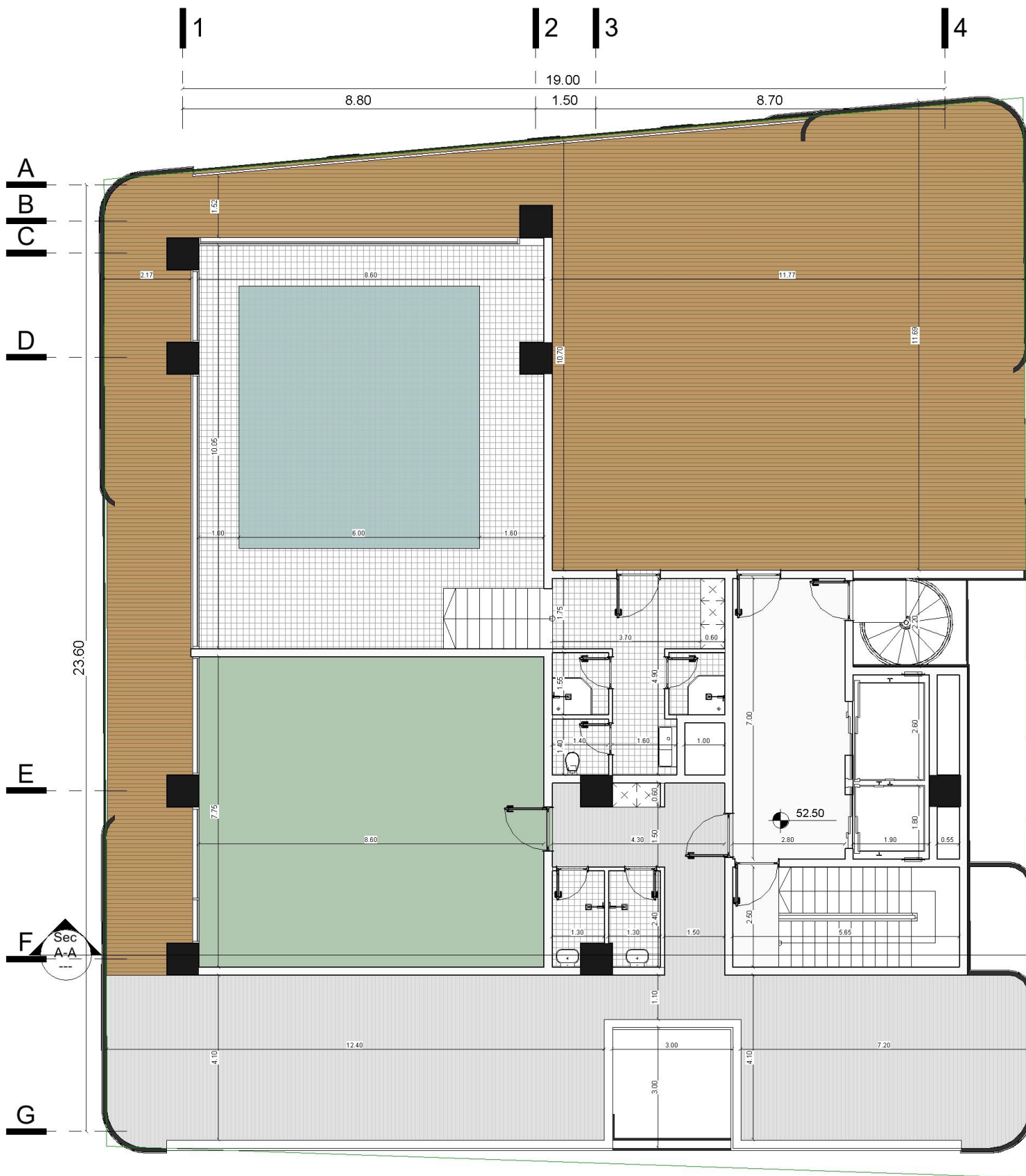
ROOF PLAN TOTAL AREA = 545 M 2
