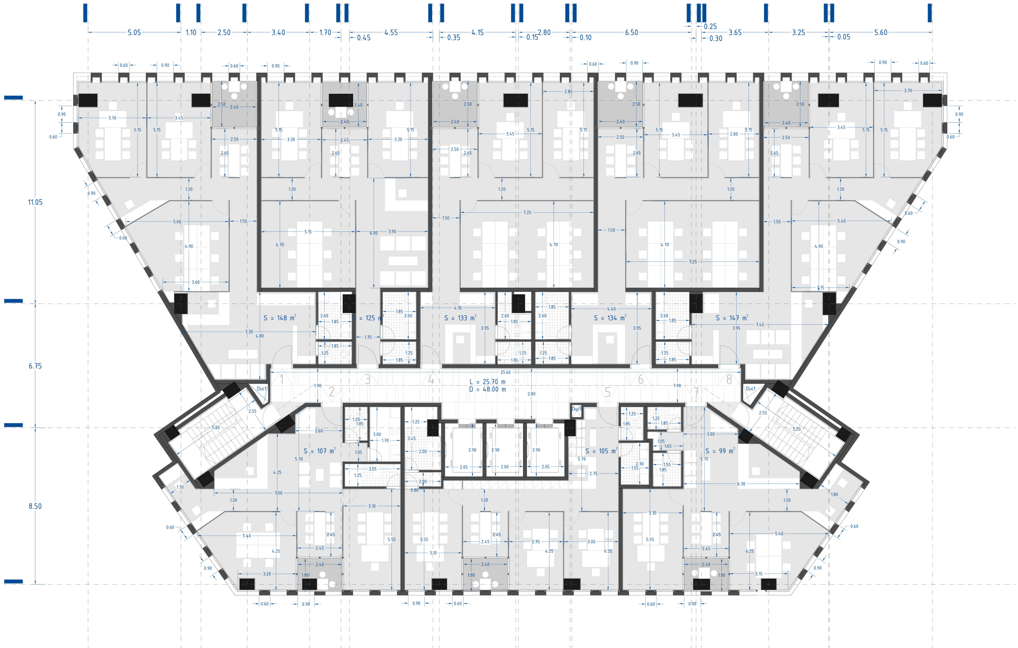
Typical Office Floor Dimension Plan
