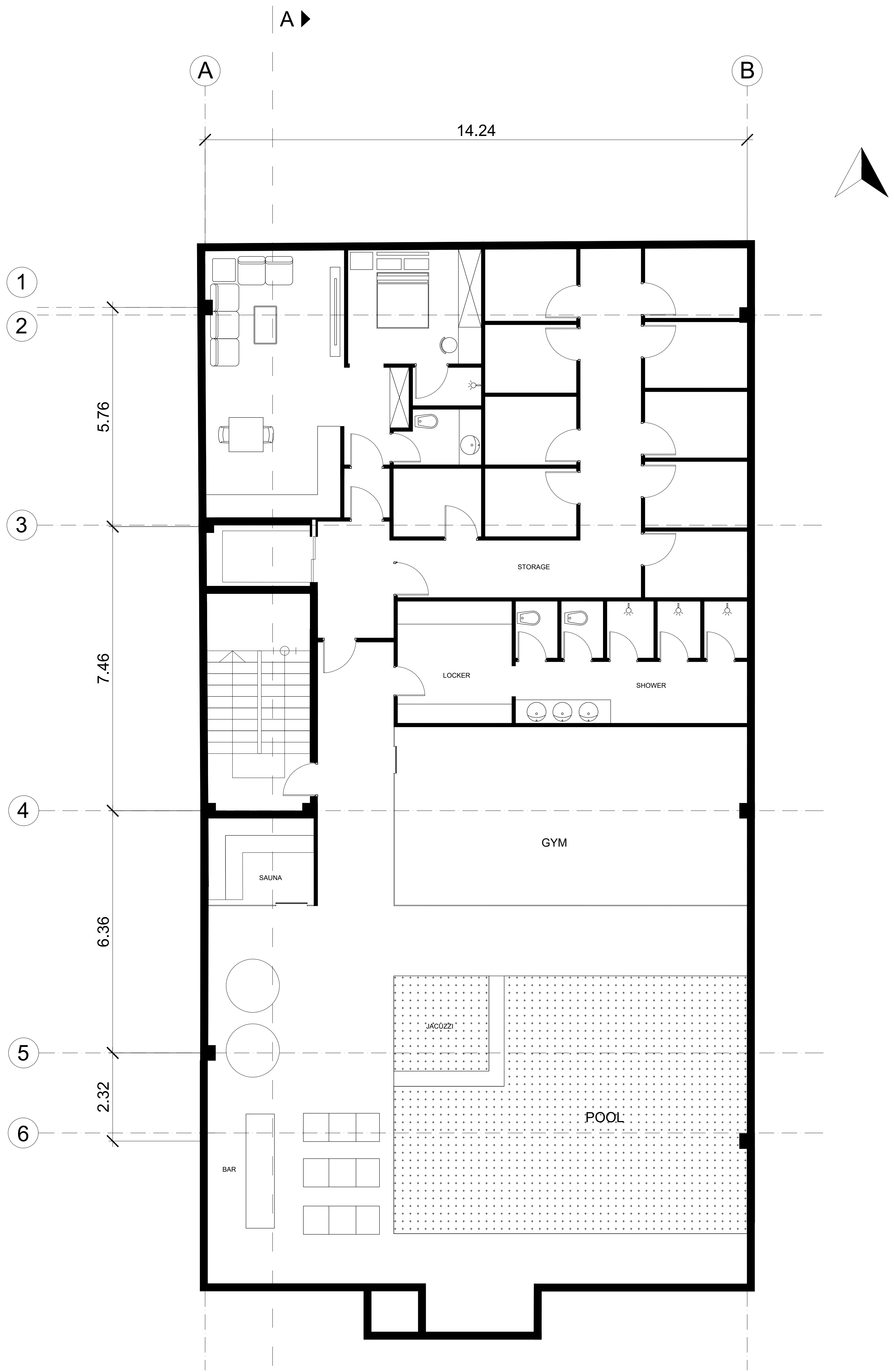
-3 FLOOR PLAN - 9.60
