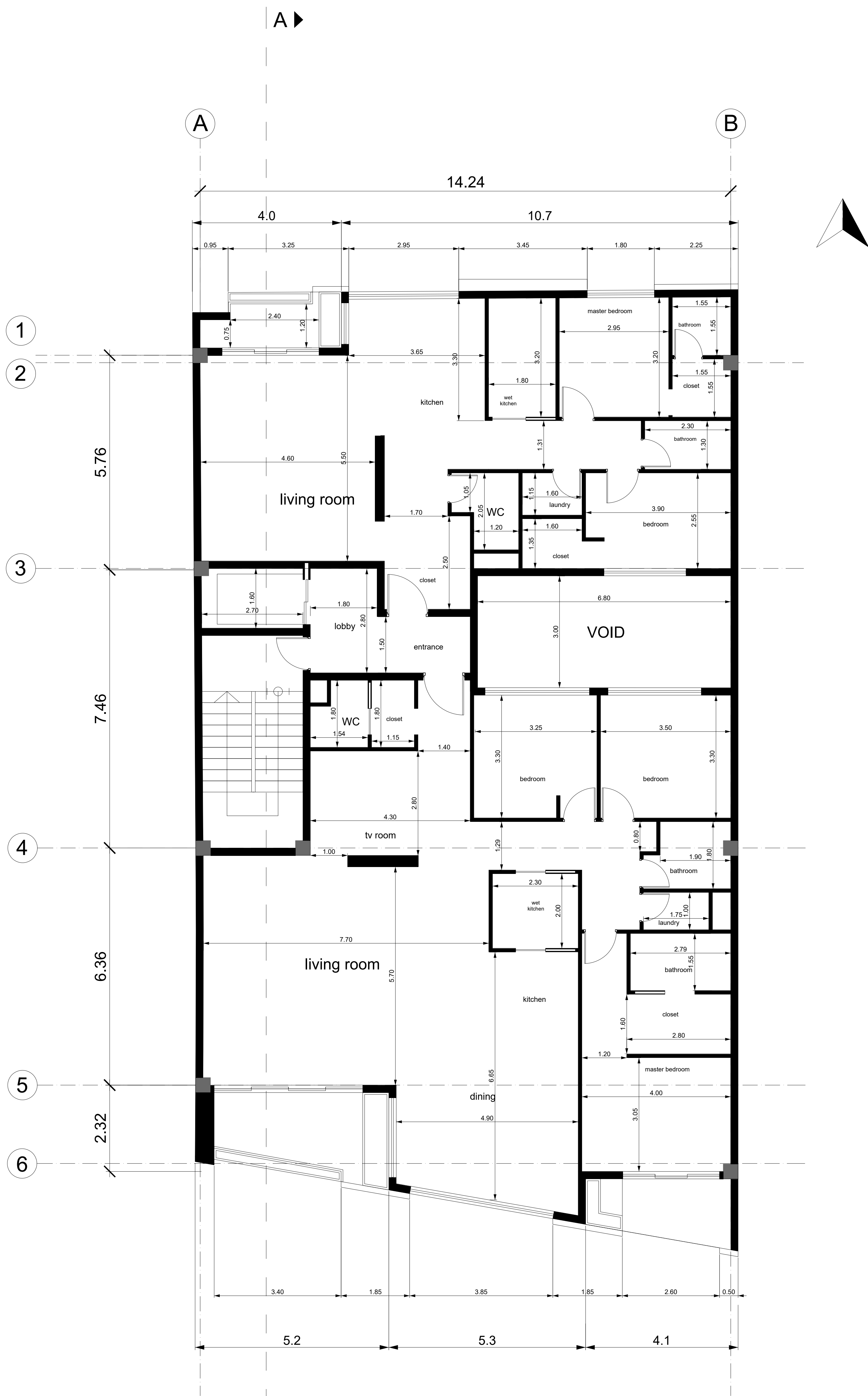
THIRD FLOOR PLAN + 13.80
