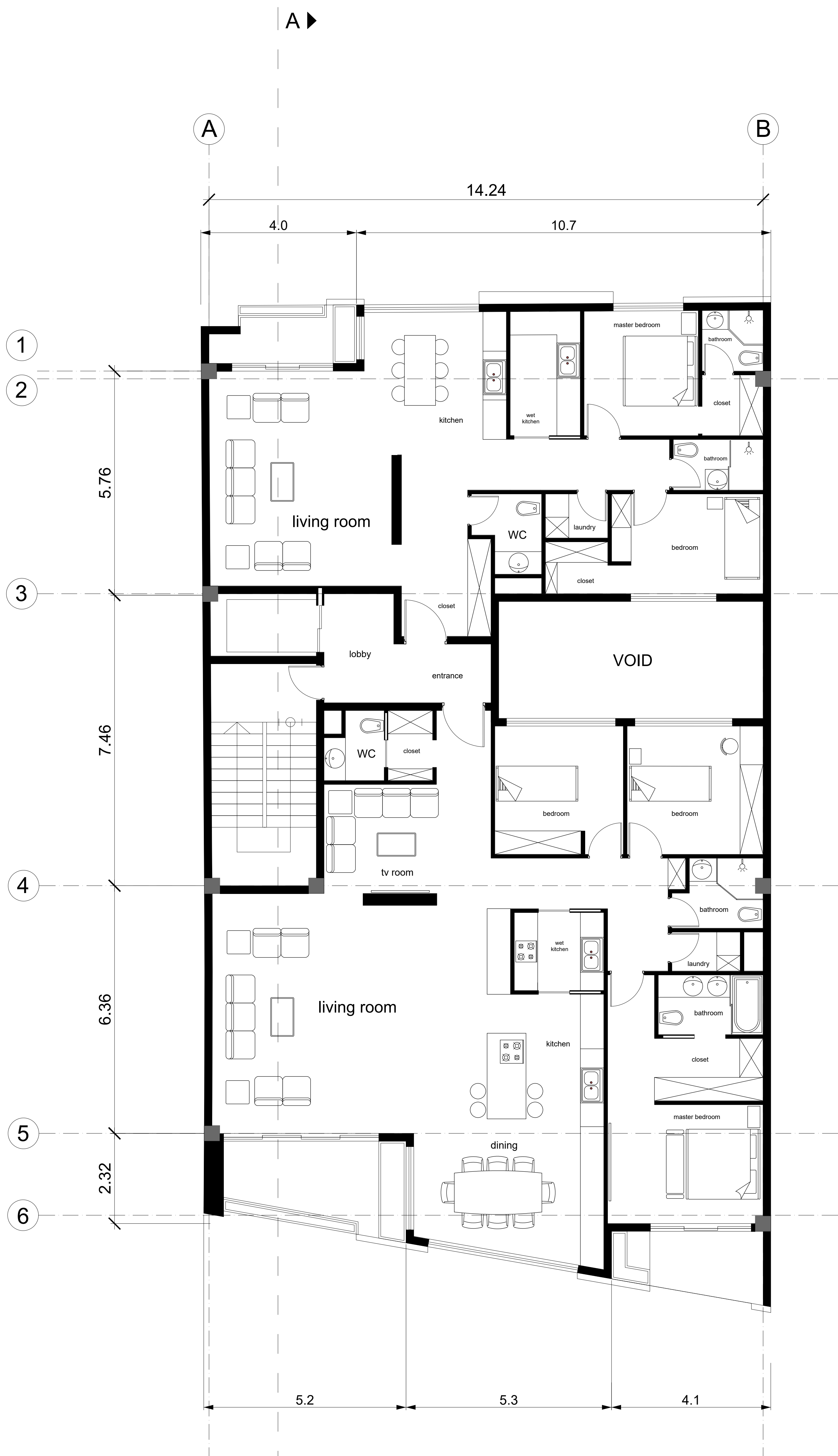
THIRD FLOOR PLAN + 13.80
