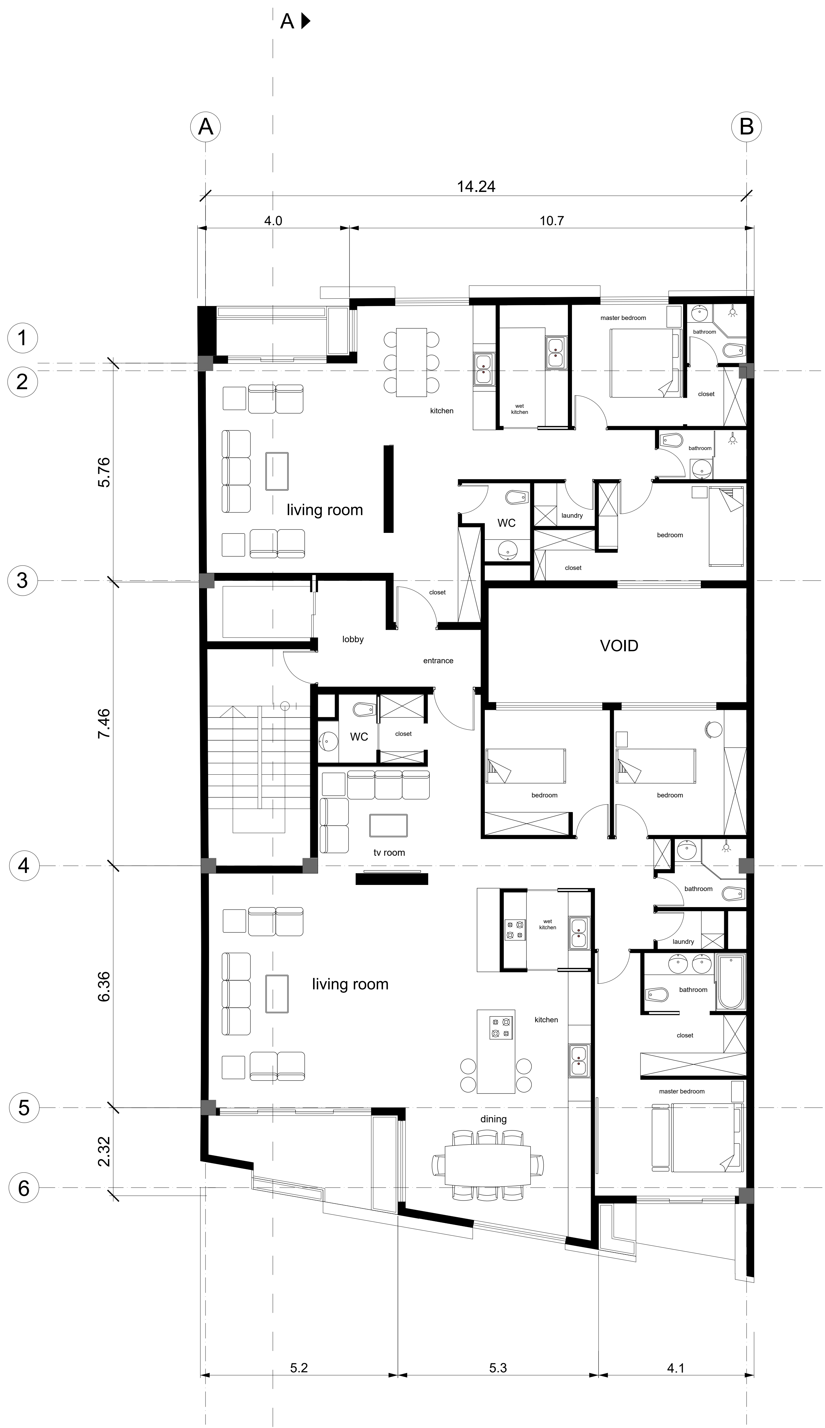
FIFTH FLOOR PLAN + 21.40
