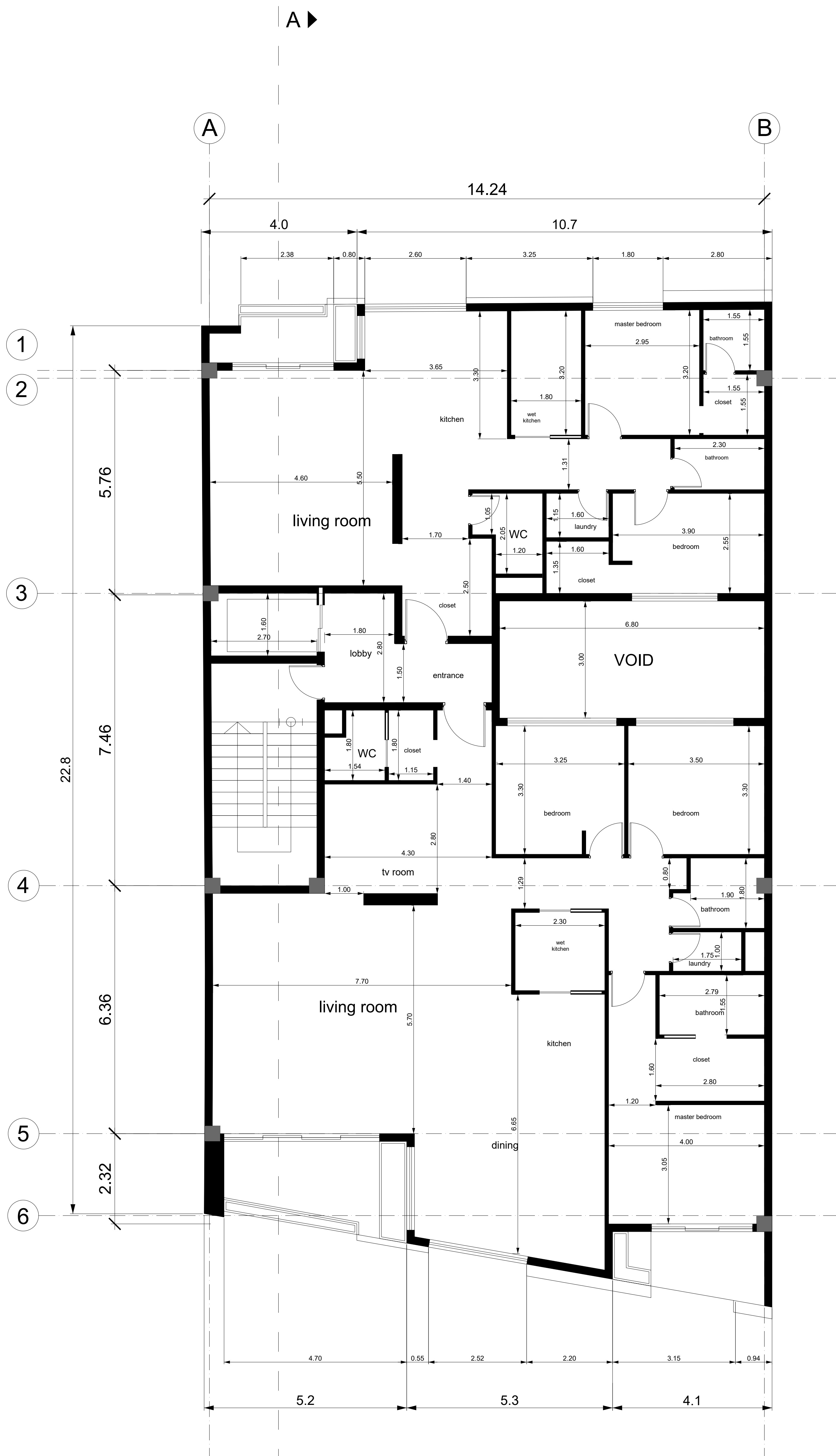
SECOND FLOOR PLAN + 10.00
