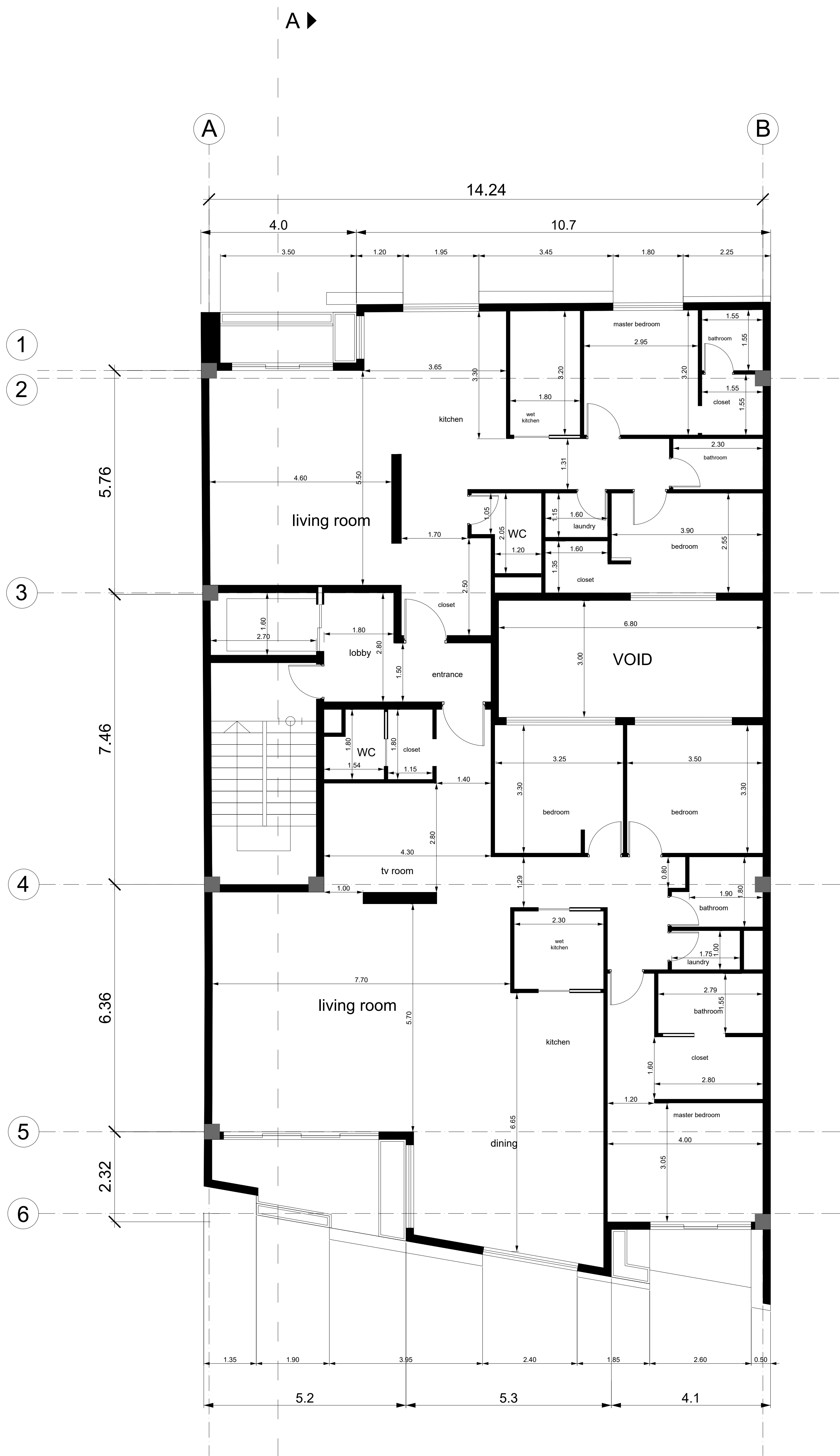
FORTH FLOOR PLAN + 17.60
