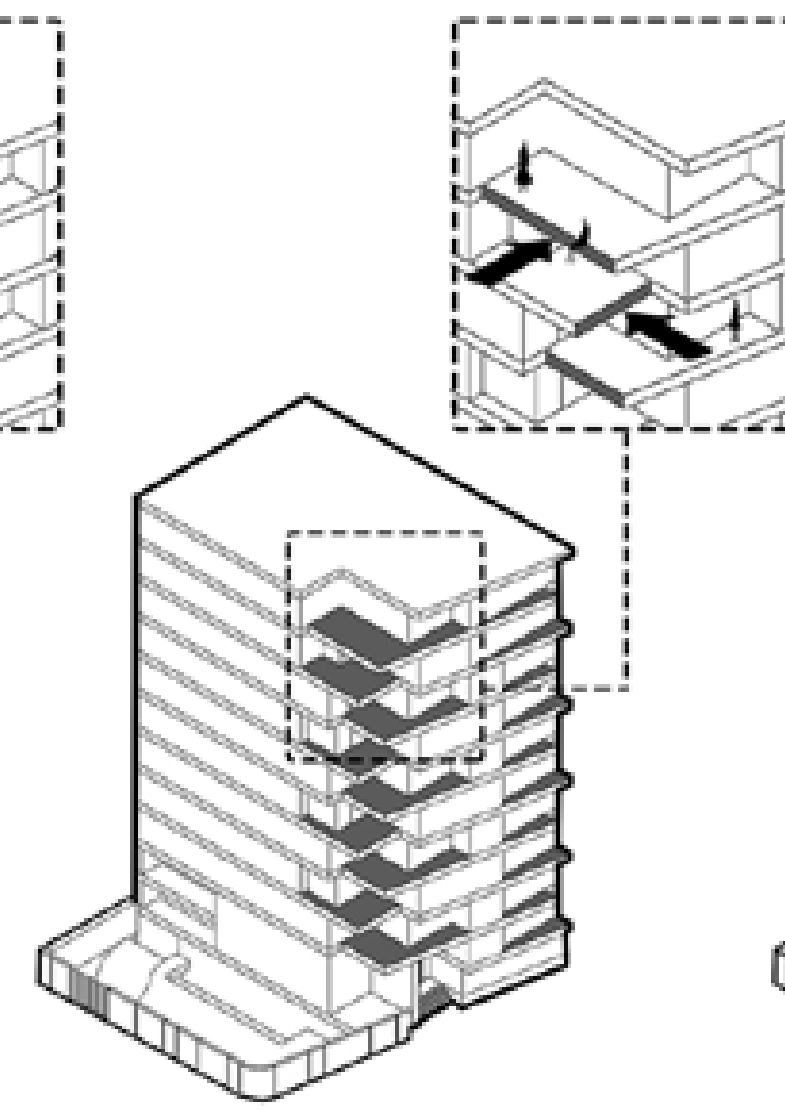
⊕ MOVING TERRACE
