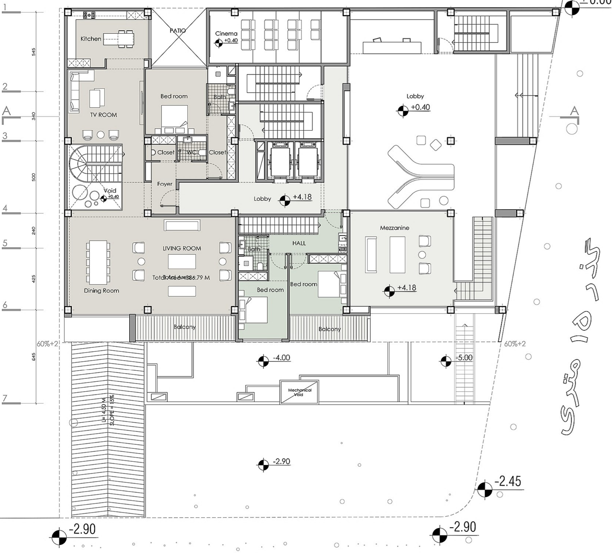
Ground Floor Plan (Mezzanine)
