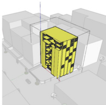
4.Edited volume
