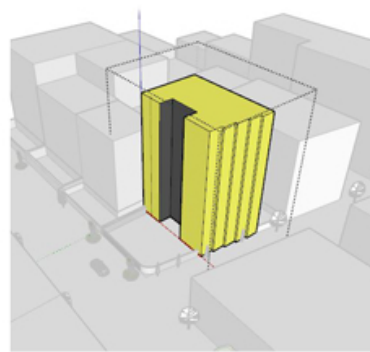
3.Shifted volume
