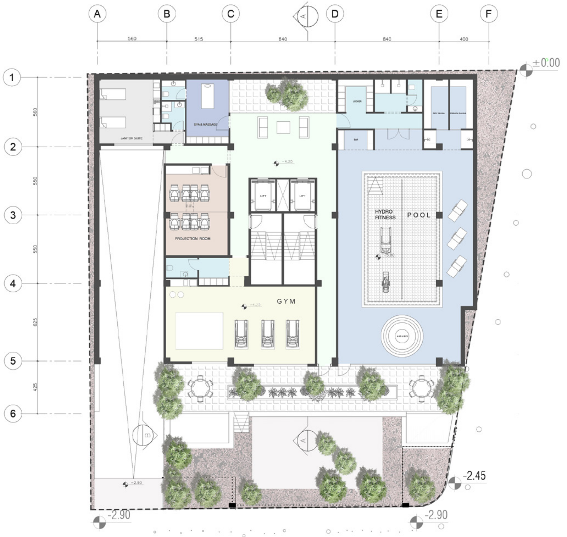
- 1 BASEMENT PLAN
