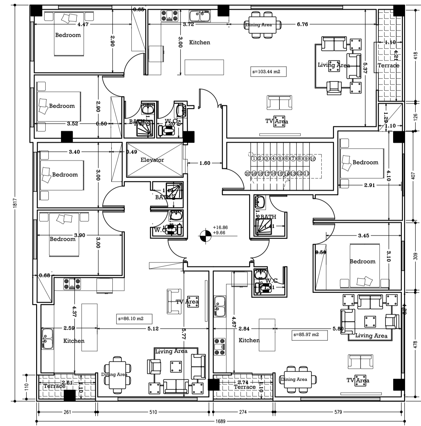
2&4 th Floor Plan
