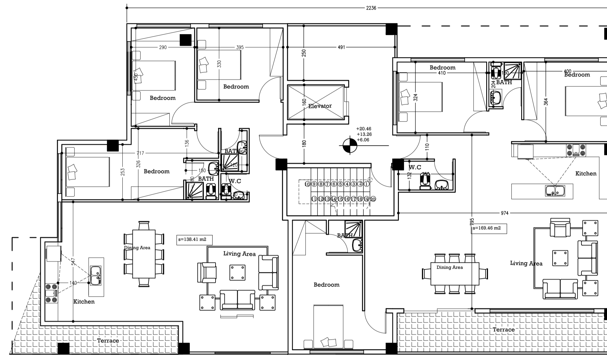
1&3 th Floor Plan
