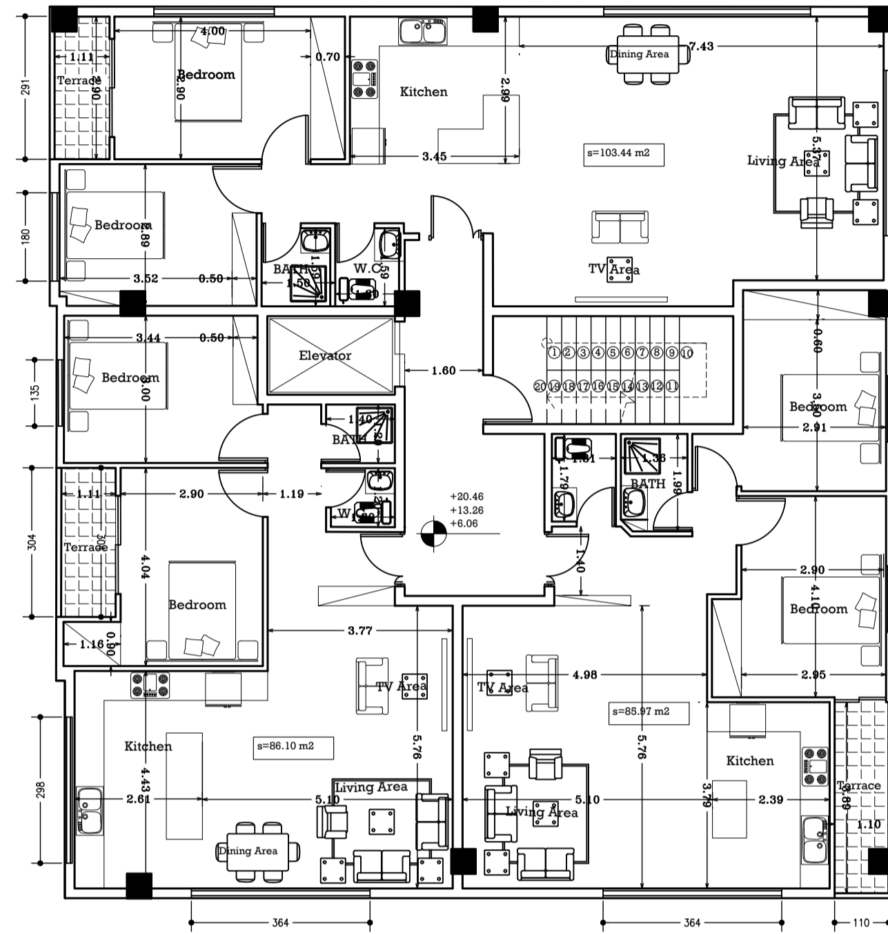
1&3&5 th Floor Plan
