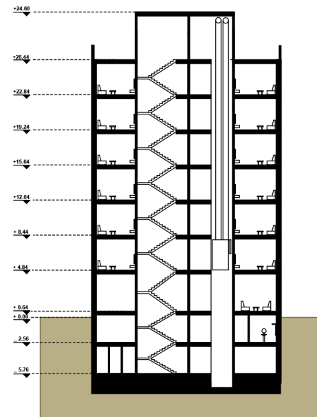
SECTION A-A SC 1/100
