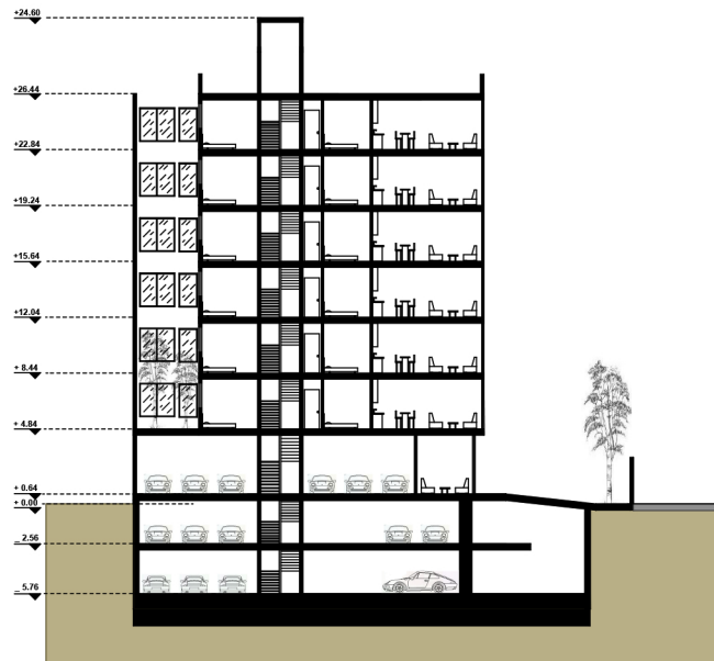
SECTION B-B SC 1/100
