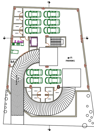
-1 BASEMENT PLAN
