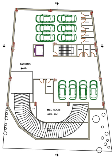
-2 BASEMENT PLAN
