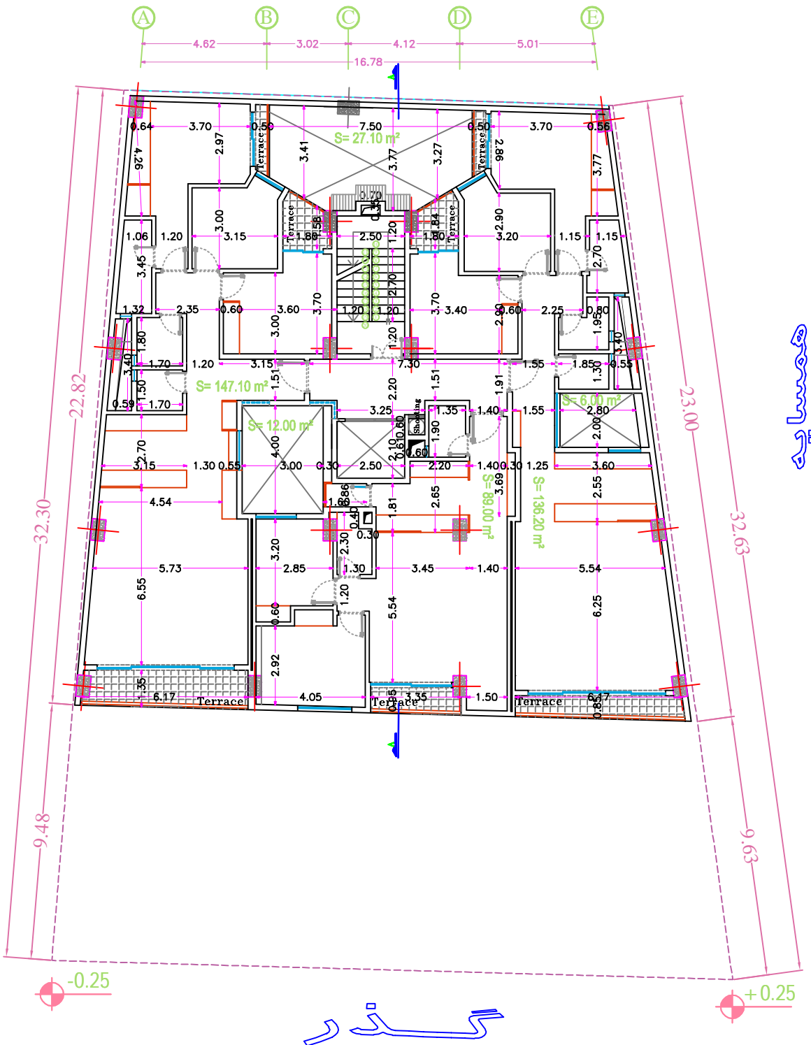
Typical Floors Plan (measurement)
