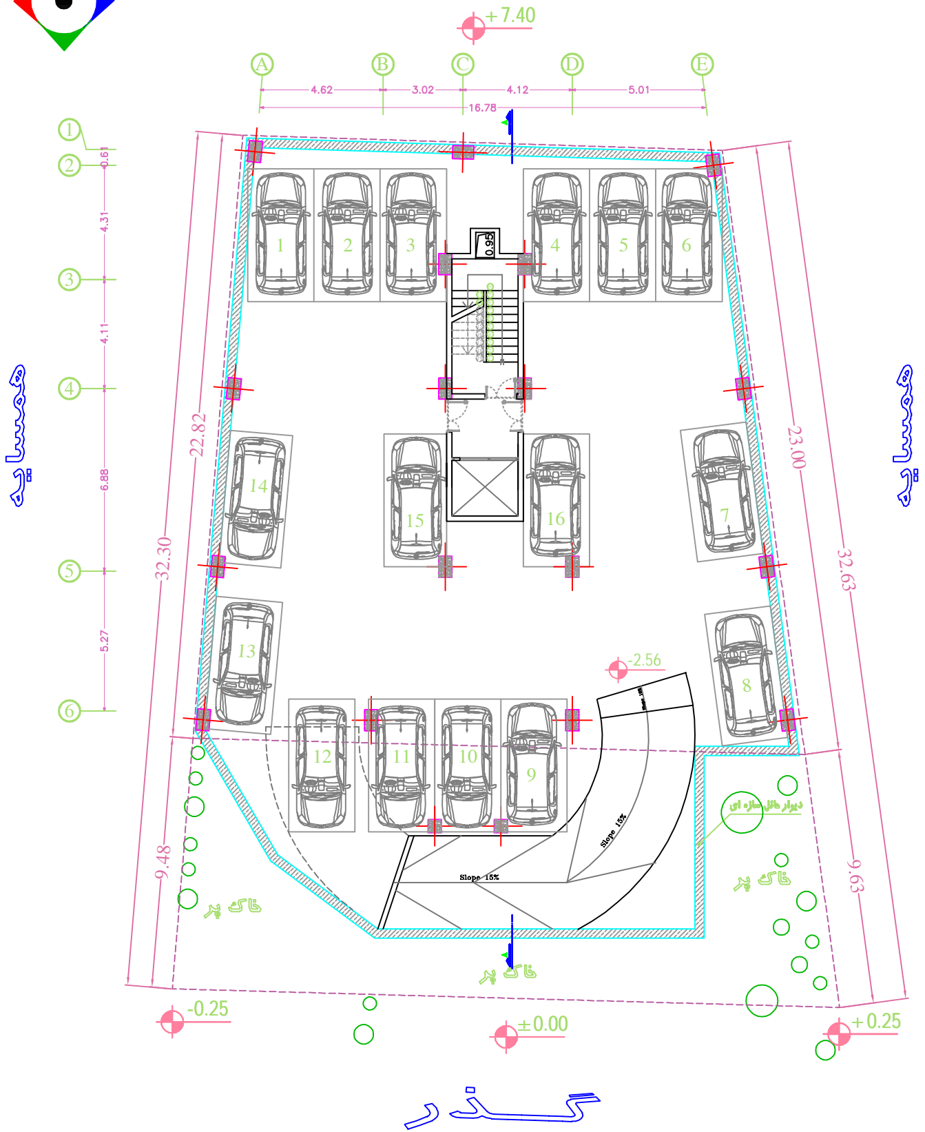
Under Ground Floor -2 (furniture)
