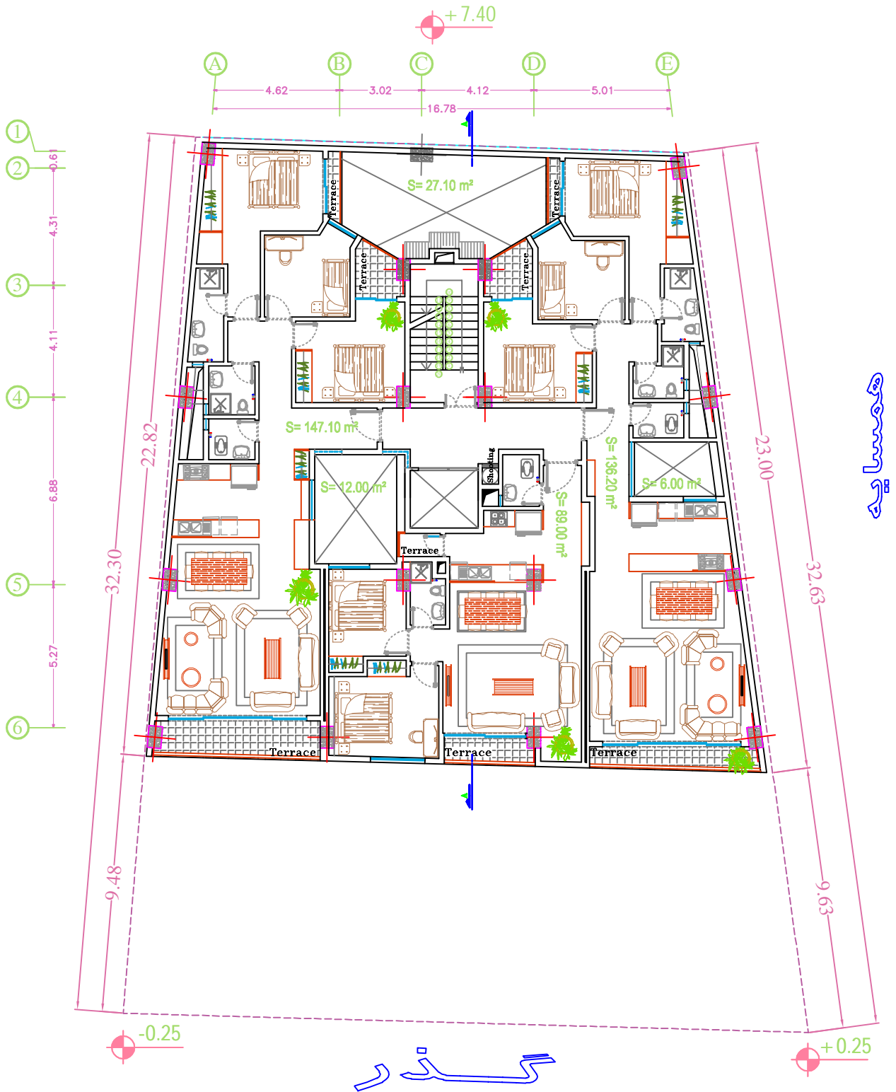
Typical Floors Plan (furniture)
