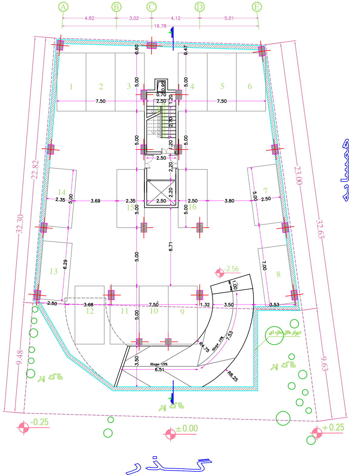
Under Ground Floor -2 (measurement)
