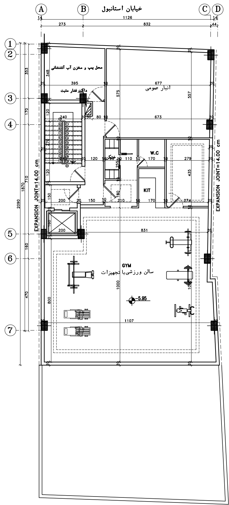
BASEMENT-2 FLOOR PLAN SC. 1:100
