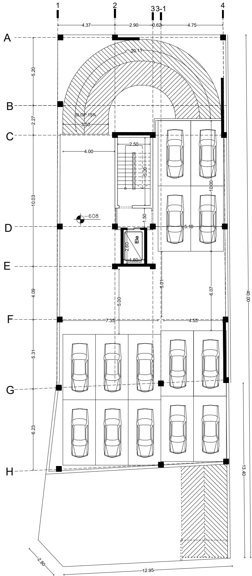
2 Under Ground floor plan
