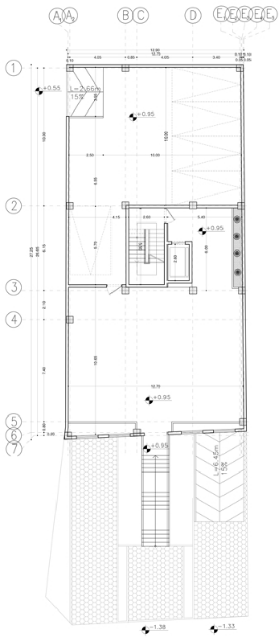
Ground Floor Plan Dimension Plan
