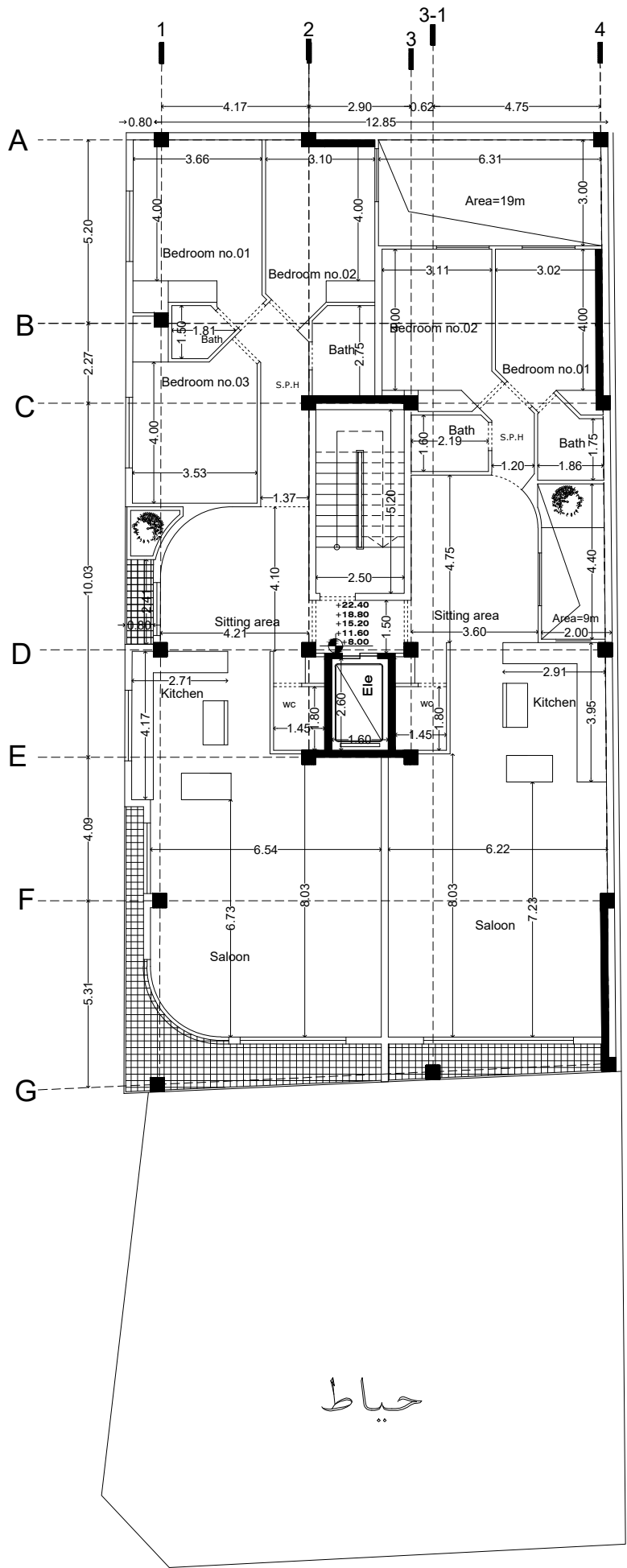
typical floors plan
