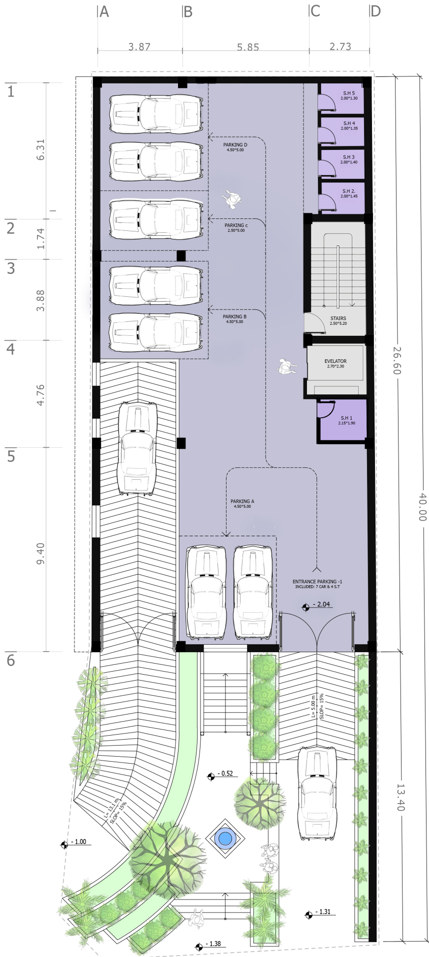
-1 FLOOR PLAN DOWLAT PROJECT L RAMP= 5 m / SLOP RAMP= 15% INCLUDED: 7 UNIT PARKING & 5 S.H
