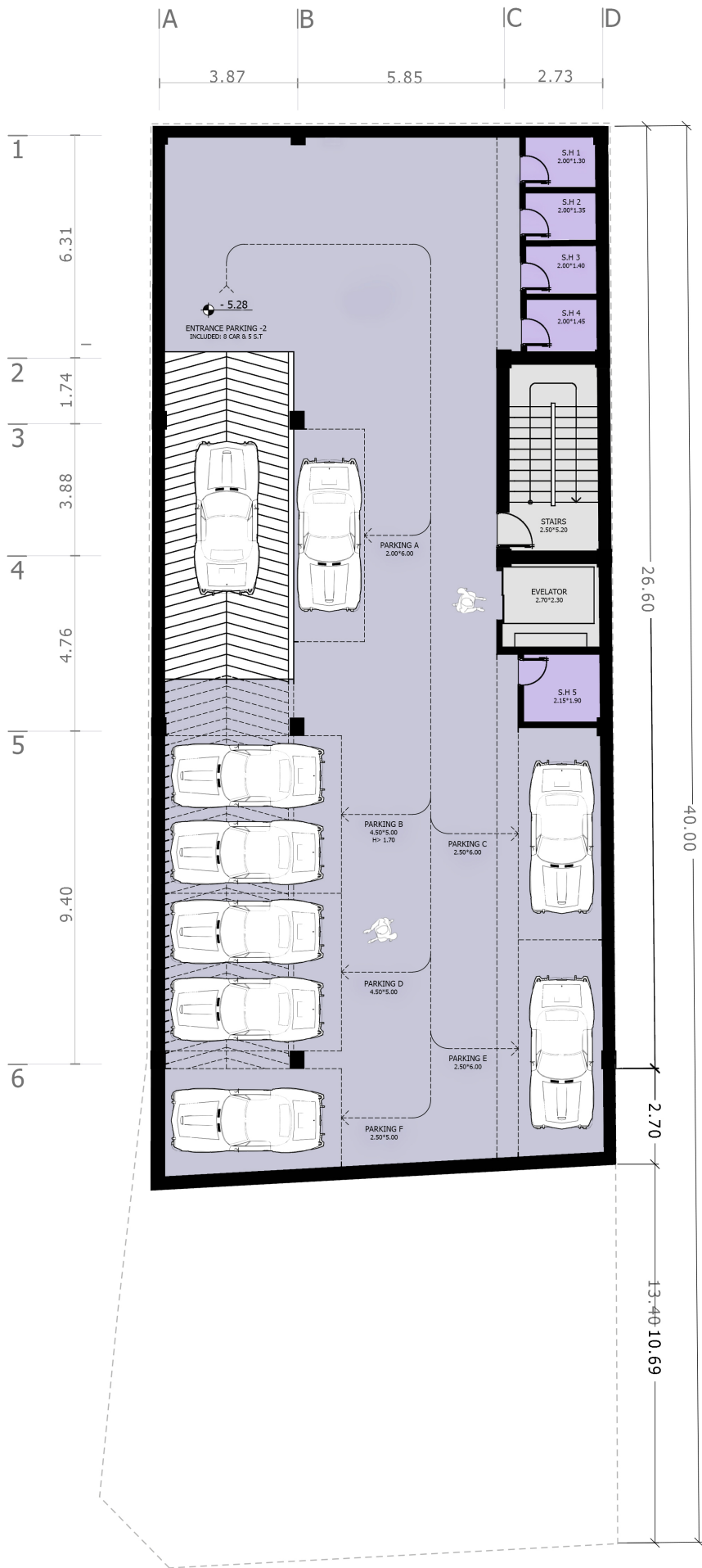
-2 FLOOR PLAN DOWLAT PROJECT L.RAMP= 28.50 m / SLOP RAMP= 15% INCLUDED: 8 UNIT PARKING & 5 S.H
