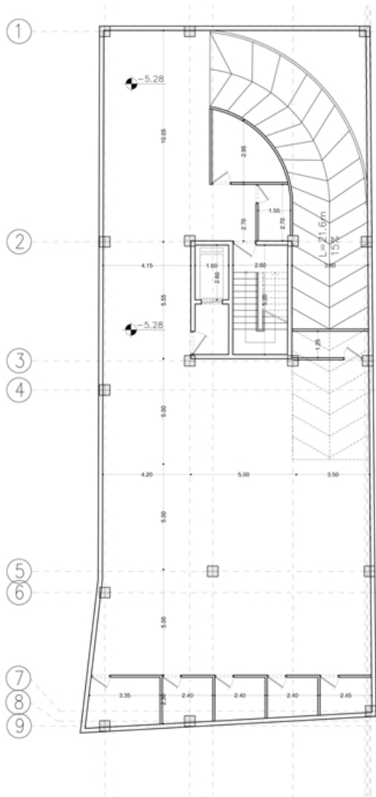
Second Basement Dimention Plan
