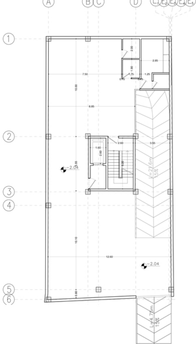
First Basement Dimension Plan
