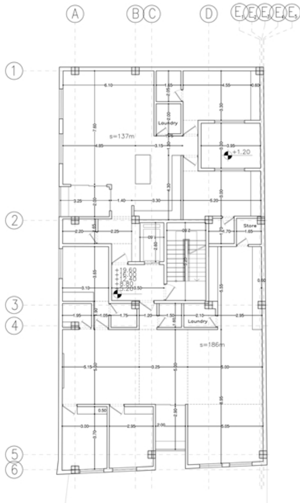
Typical Dimention Plan
