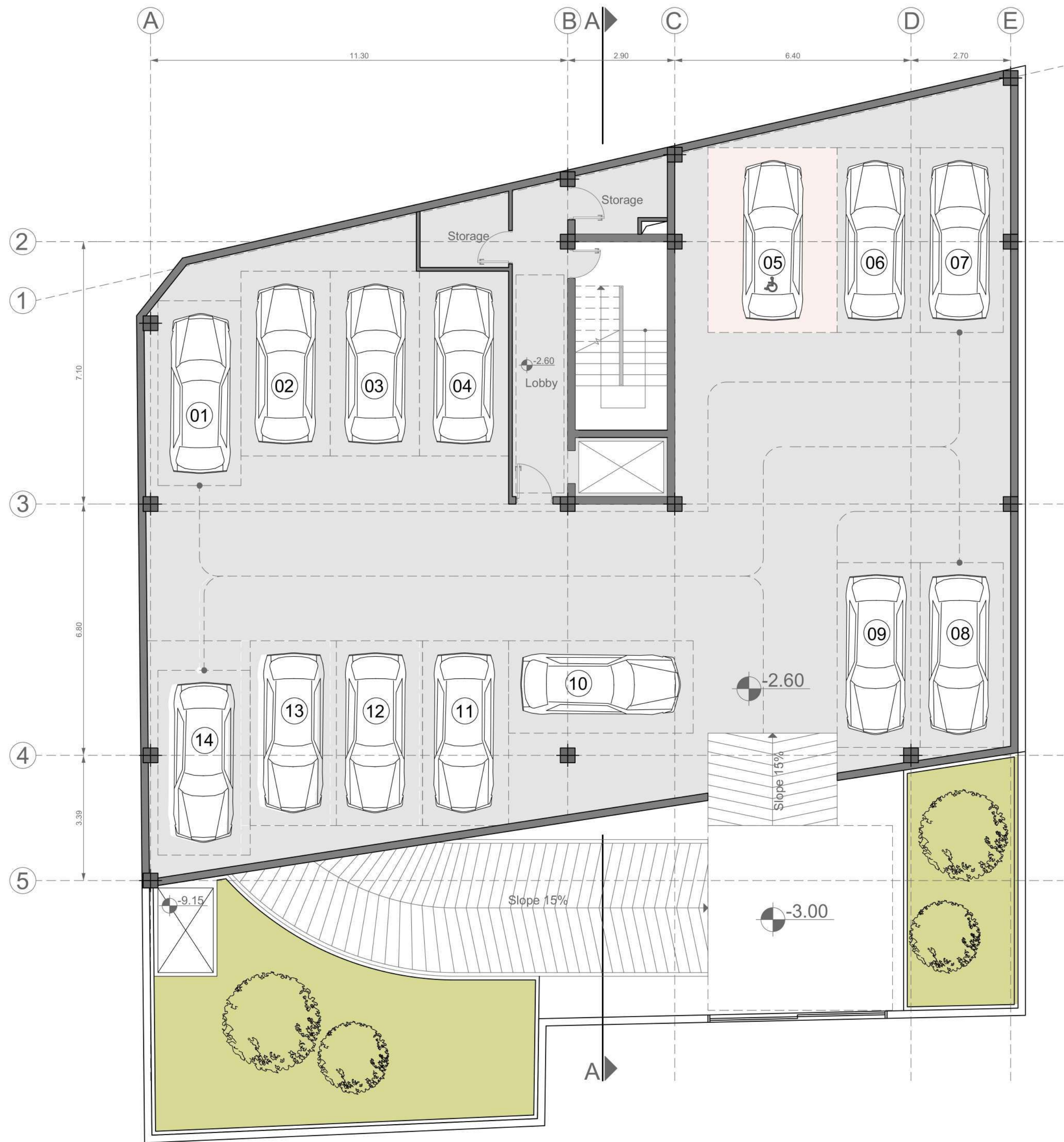
Parking -1 Floor Plan
