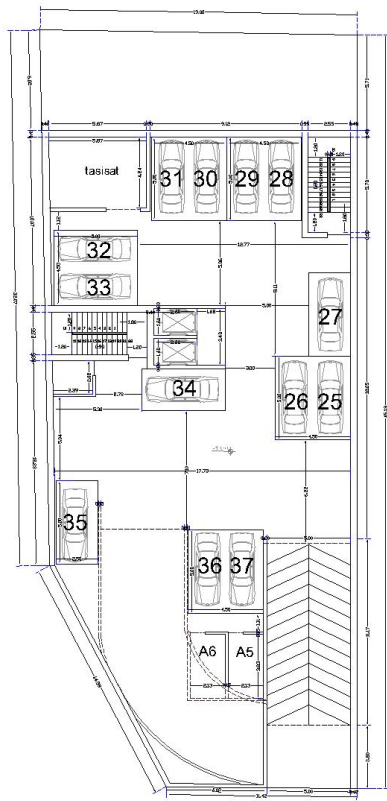
basement -3
