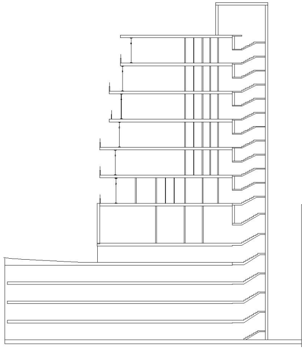
section 1-1
