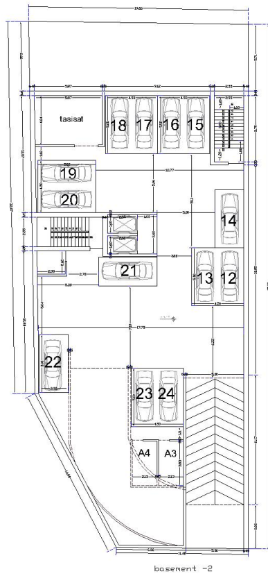
basement -2
